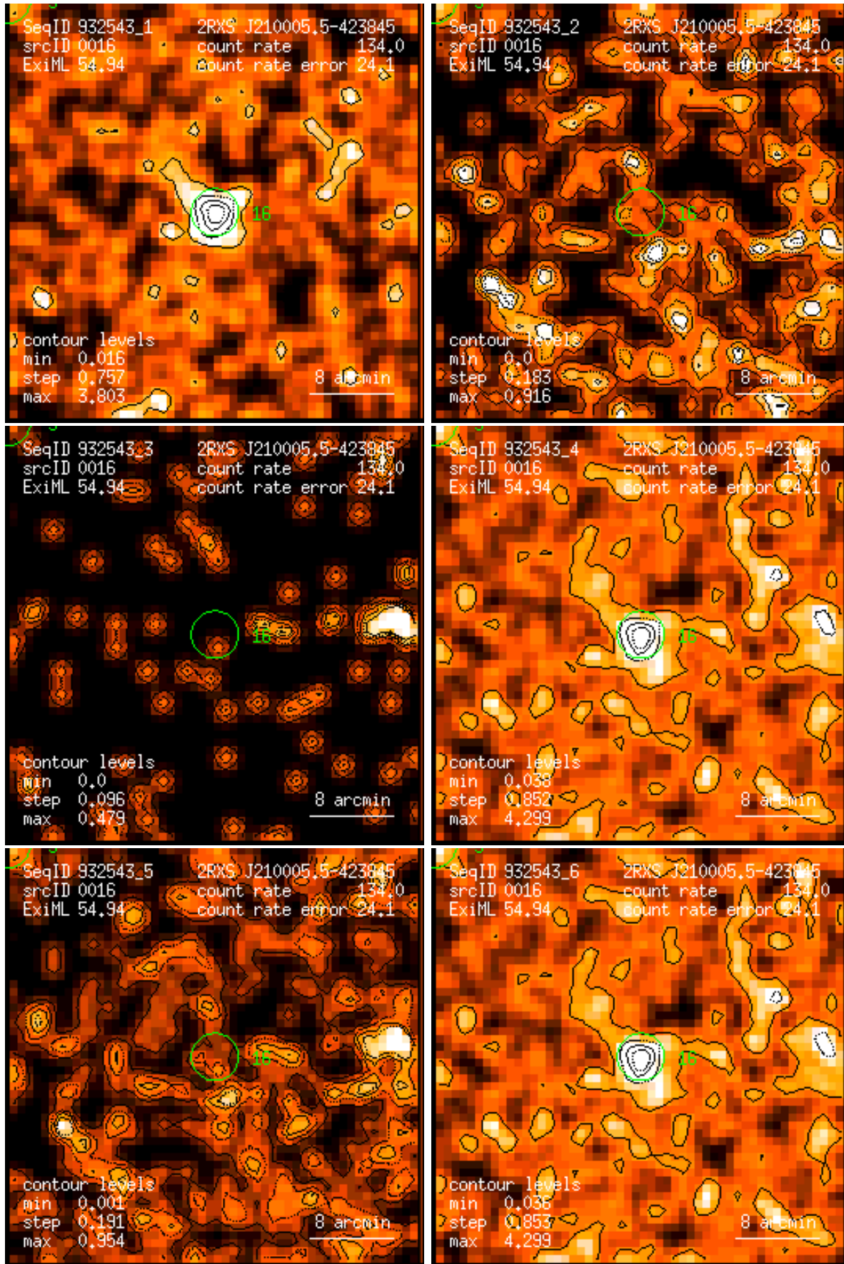
Figure 16: RASS 932543: detection 0016: band rate images, Gaussian filter: (1) PSPC channels 11 – 41, (2) 52 – 90, (3) 91 – 201, (4) 11 – 235, (5) 52 – 201, (6) 11 – 201. Broad band rates in counts/ks. Band rate contour levels in counts/ks/arcmin 2 .
