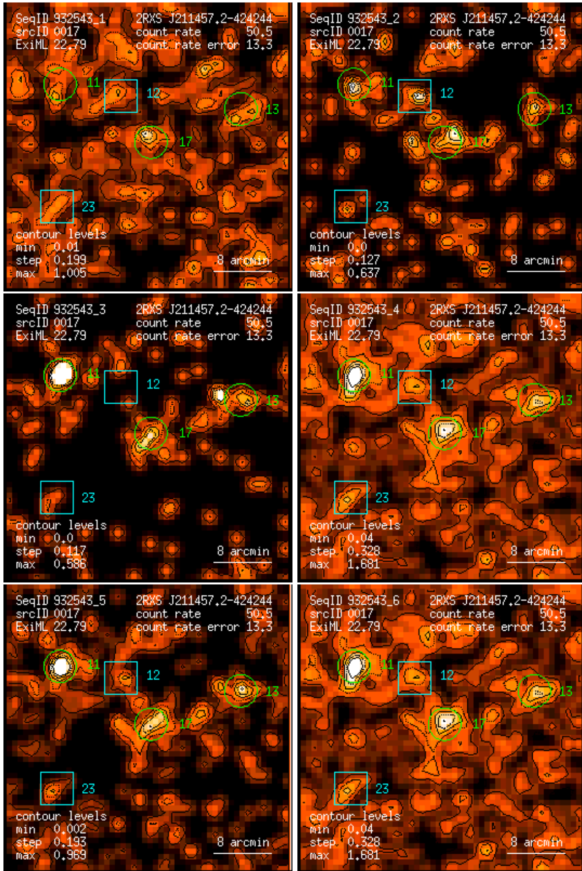
Figure 17: RASS 932543: detection 0017: band rate images, Gaussian filter: (1) PSPC channels 11 – 41, (2) 52 – 90, (3) 91 – 201, (4) 11 – 235, (5) 52 – 201, (6) 11 – 201. Broad band rates in counts/ks. Band rate contour levels in counts/ks/arcmin 2 .
