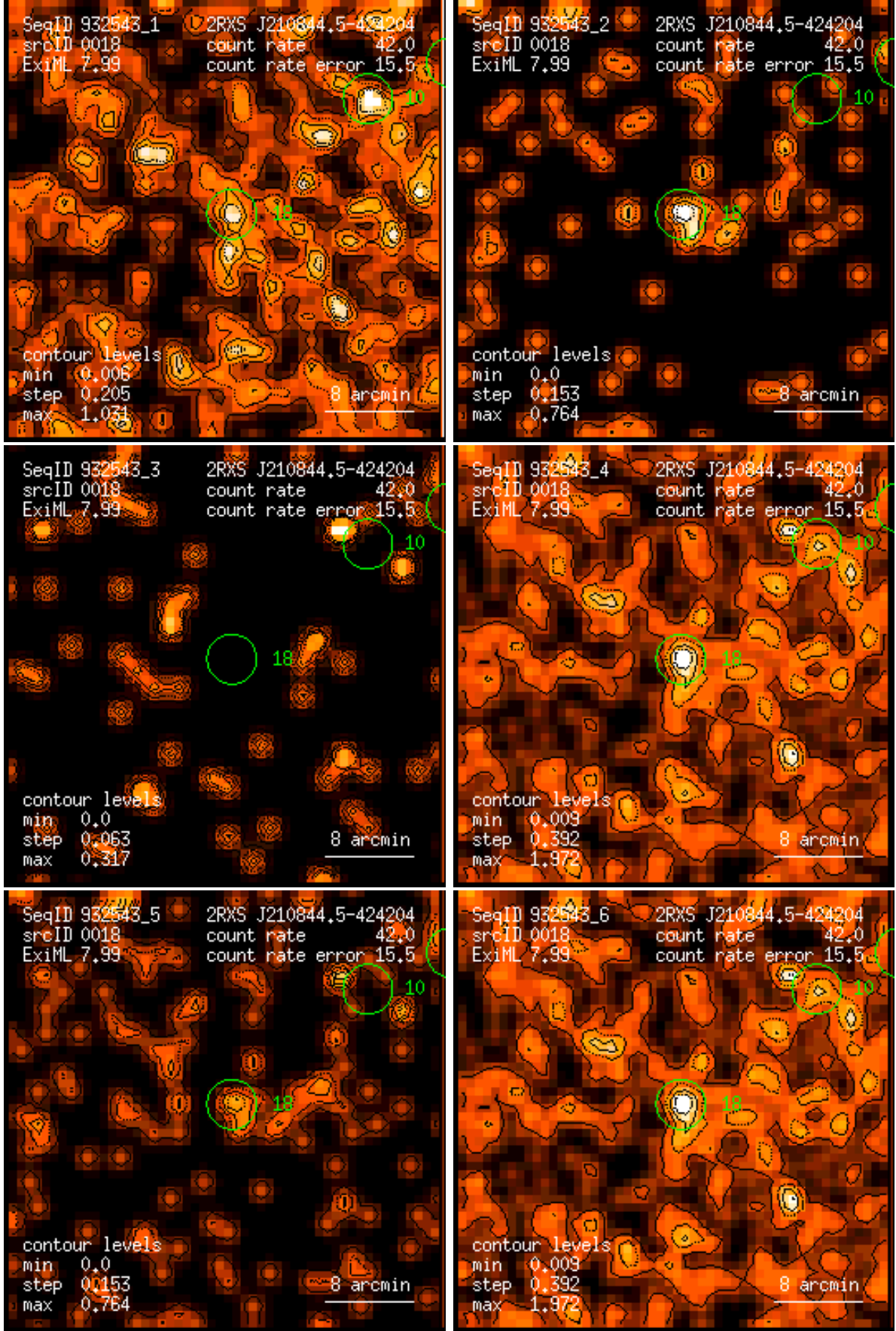
Figure 18: RASS 932543: detection 0018: band rate images, Gaussian filter: (1) PSPC channels 11 – 41, (2) 52 – 90, (3) 91 – 201, (4) 11 – 235, (5) 52 – 201, (6) 11 – 201. Broad band rates in counts/ks. Band rate contour levels in counts/ks/arcmin 2 .
