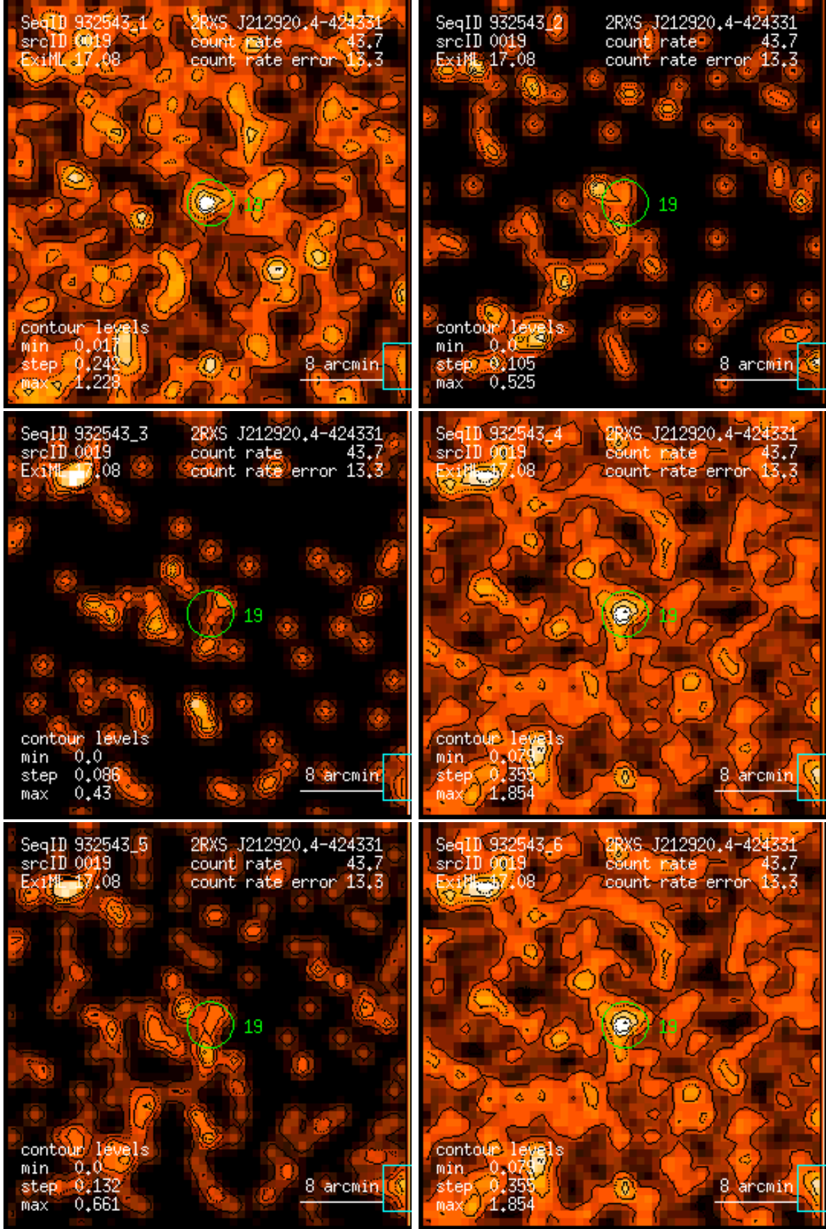
Figure 19: RASS 932543: detection 0019: band rate images, Gaussian filter: (1) PSPC channels 11 – 41, (2) 52 – 90, (3) 91 – 201, (4) 11 – 235, (5) 52 – 201, (6) 11 – 201. Broad band rates in counts/ks. Band rate contour levels in counts/ks/arcmin 2 .
