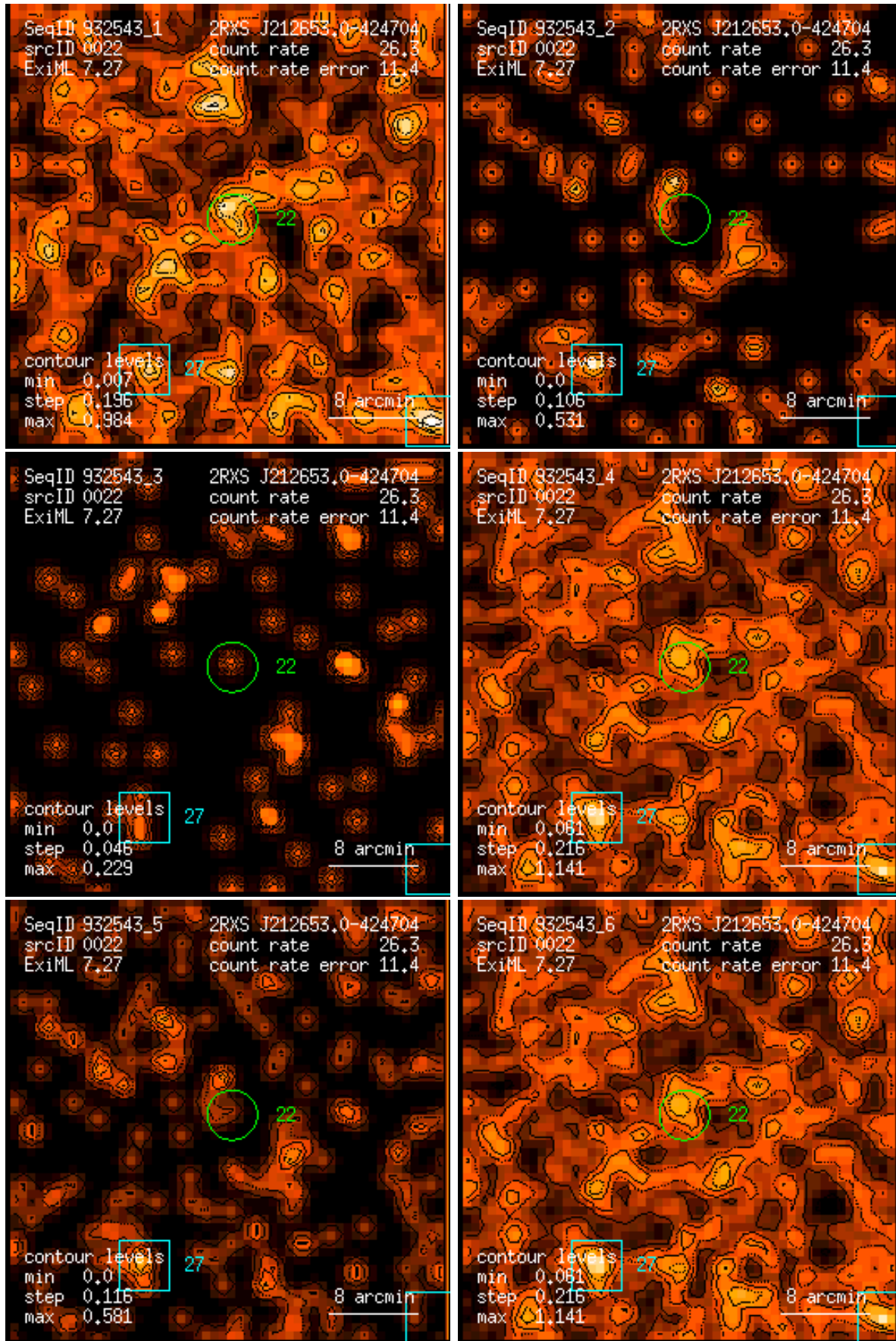
Figure 22: RASS 932543: detection 0022: band rate images, Gaussian filter: (1) PSPC channels 11 – 41, (2) 52 – 90, (3) 91 – 201, (4) 11 – 235, (5) 52 – 201, (6) 11 – 201. Broad band rates in counts/ks. Band rate contour levels in counts/ks/arcmin 2 .
