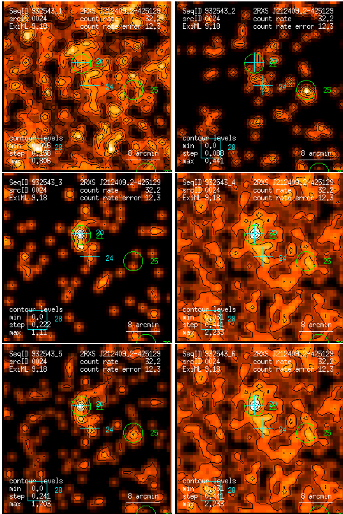
Figure 24: RASS 932543: detection 0024: band rate images, Gaussian filter: (1) PSPC channels 11 – 41, (2) 52 – 90, (3) 91 – 201, (4) 11 – 235, (5) 52 – 201, (6) 11 – 201. Broad band rates in counts/ks. Band rate contour levels in counts/ks/arcmin 2 .
