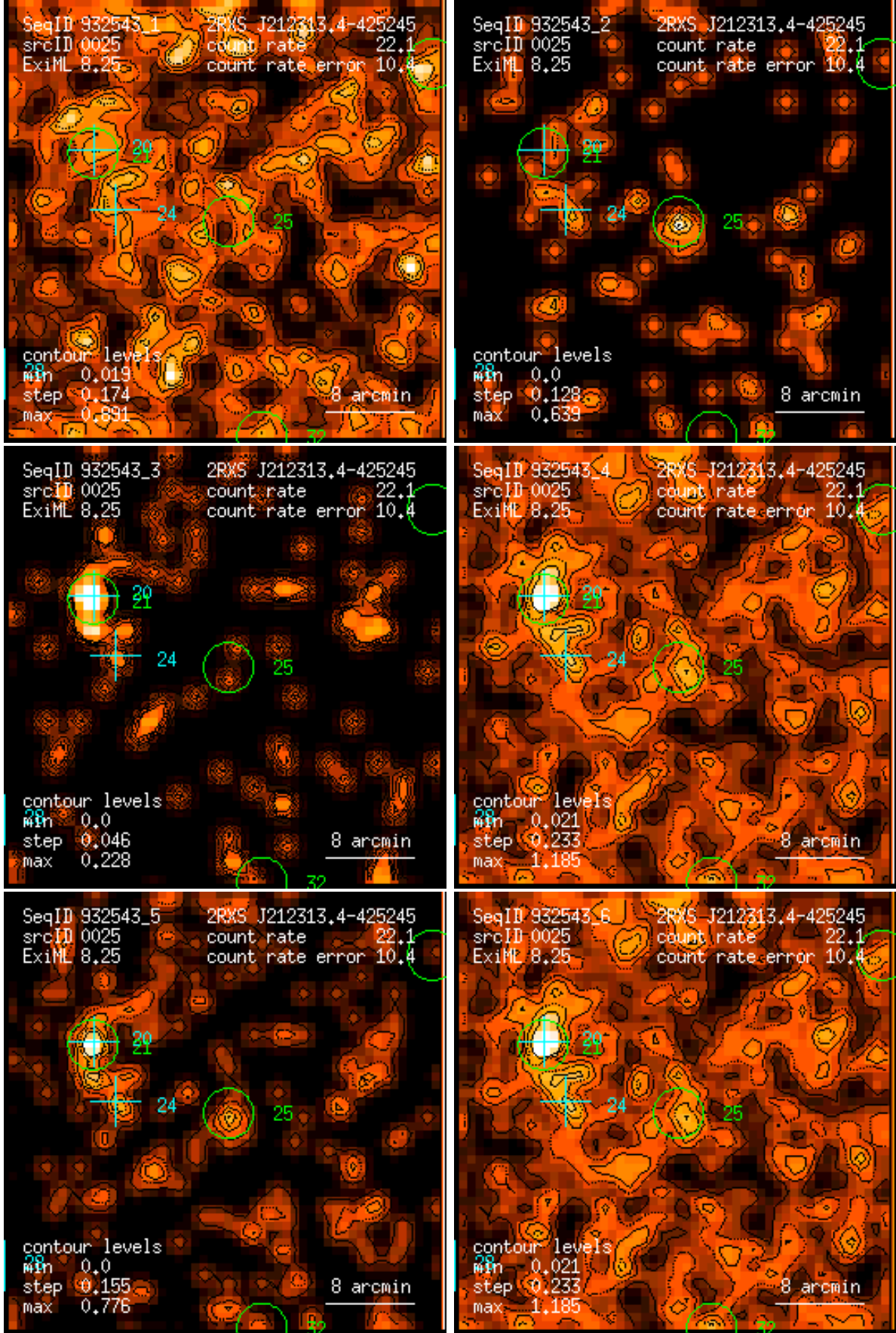
Figure 25: RASS 932543: detection 0025: band rate images, Gaussian filter: (1) PSPC channels 11 – 41, (2) 52 – 90, (3) 91 – 201, (4) 11 – 235, (5) 52 – 201, (6) 11 – 201. Broad band rates in counts/ks. Band rate contour levels in counts/ks/arcmin 2 .
