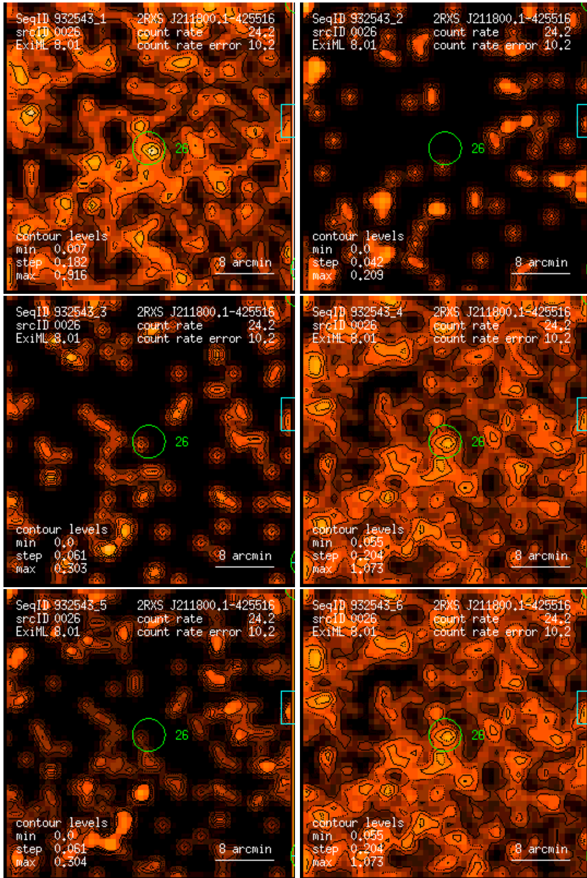
Figure 26: RASS 932543: detection 0026: band rate images, Gaussian filter: (1) PSPC channels 11 – 41, (2) 52 – 90, (3) 91 – 201, (4) 11 – 235, (5) 52 – 201, (6) 11 – 201. Broad band rates in counts/ks. Band rate contour levels in counts/ks/arcmin 2 .
