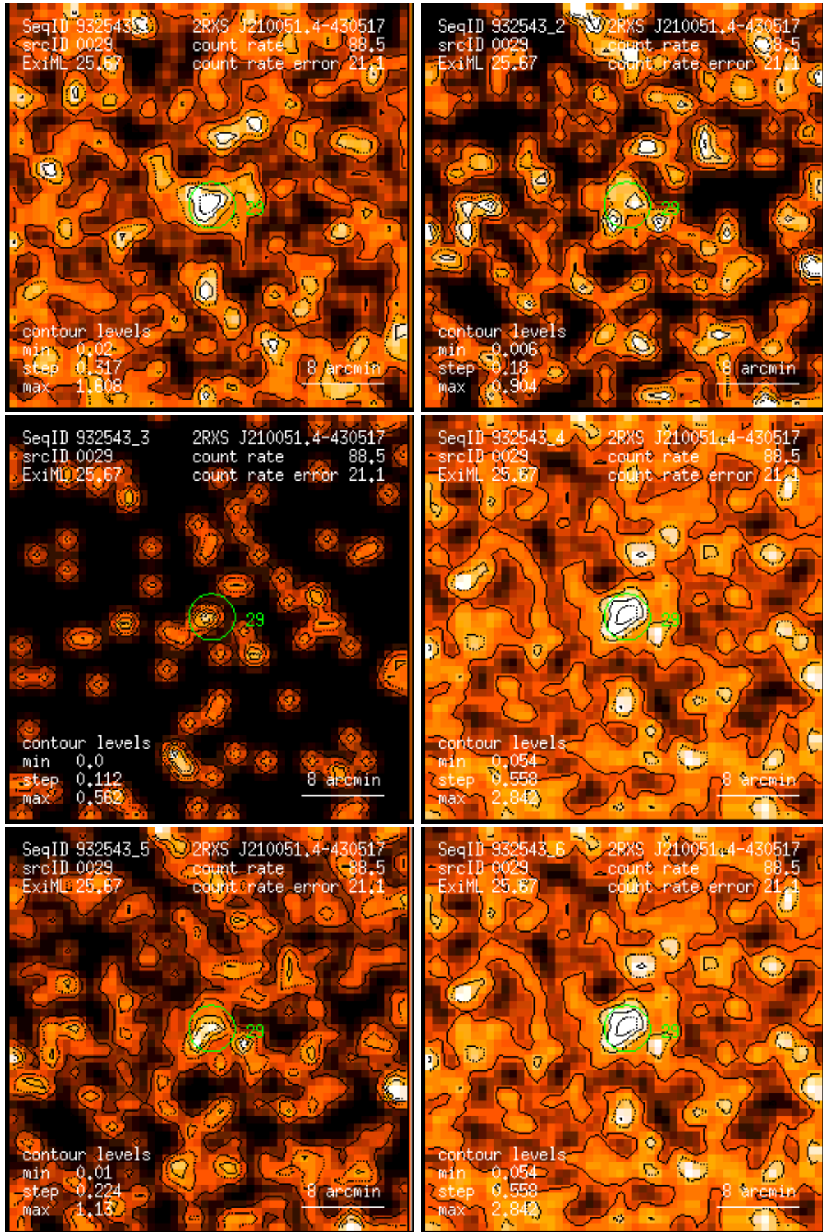
Figure 29: RASS 932543: detection 0029: band rate images, Gaussian filter: (1) PSPC channels 11 – 41, (2) 52 – 90, (3) 91 – 201, (4) 11 – 235, (5) 52 – 201, (6) 11 – 201. Broad band rates in counts/ks. Band rate contour levels in counts/ks/arcmin 2 .
