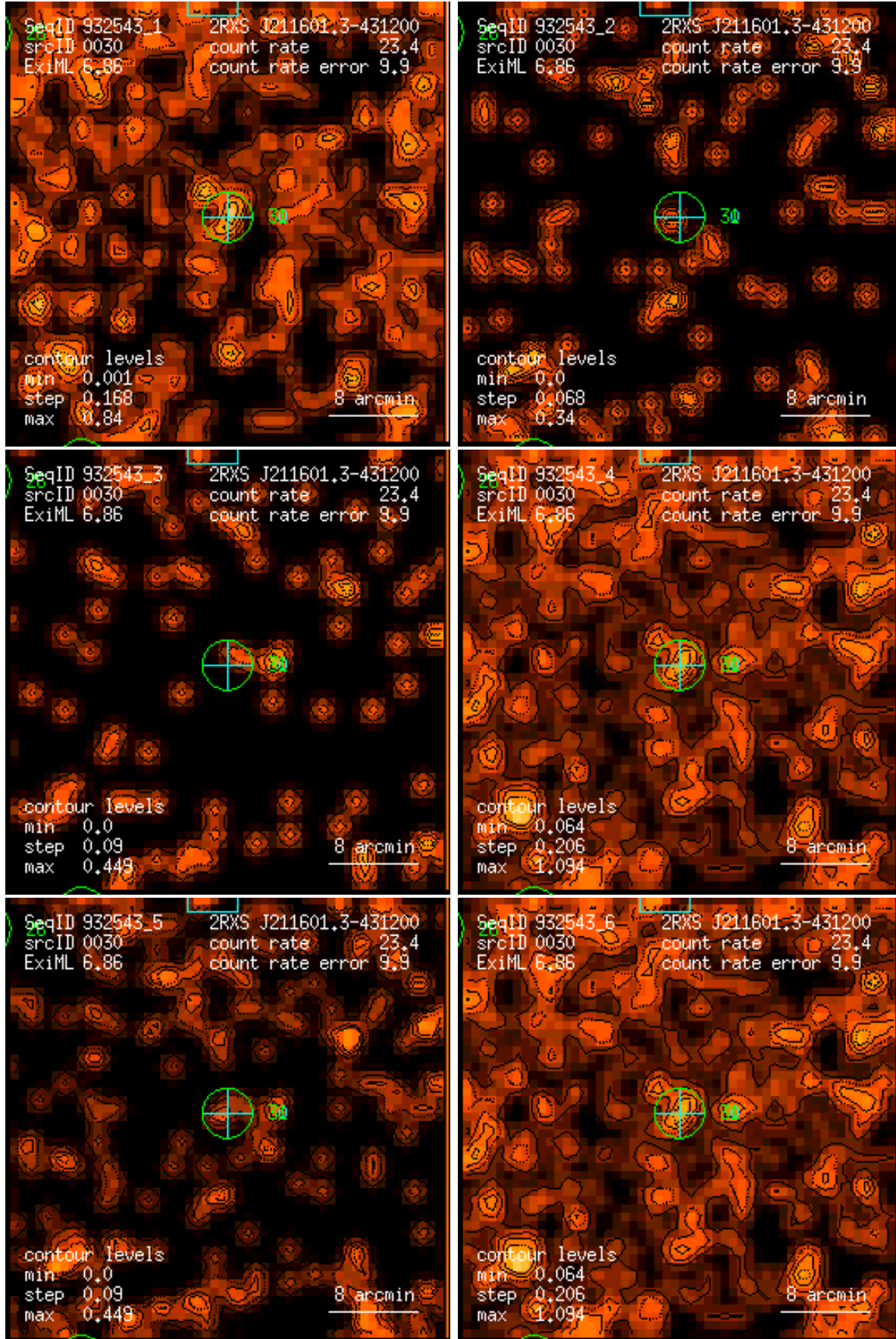
Figure 30: RASS 932543: detection 0030: band rate images, Gaussian filter: (1) PSPC channels 11 – 41, (2) 52 – 90, (3) 91 – 201, (4) 11 – 235, (5) 52 – 201, (6) 11 – 201. Broad band rates in counts/ks. Band rate contour levels in counts/ks/arcmin 2 .
