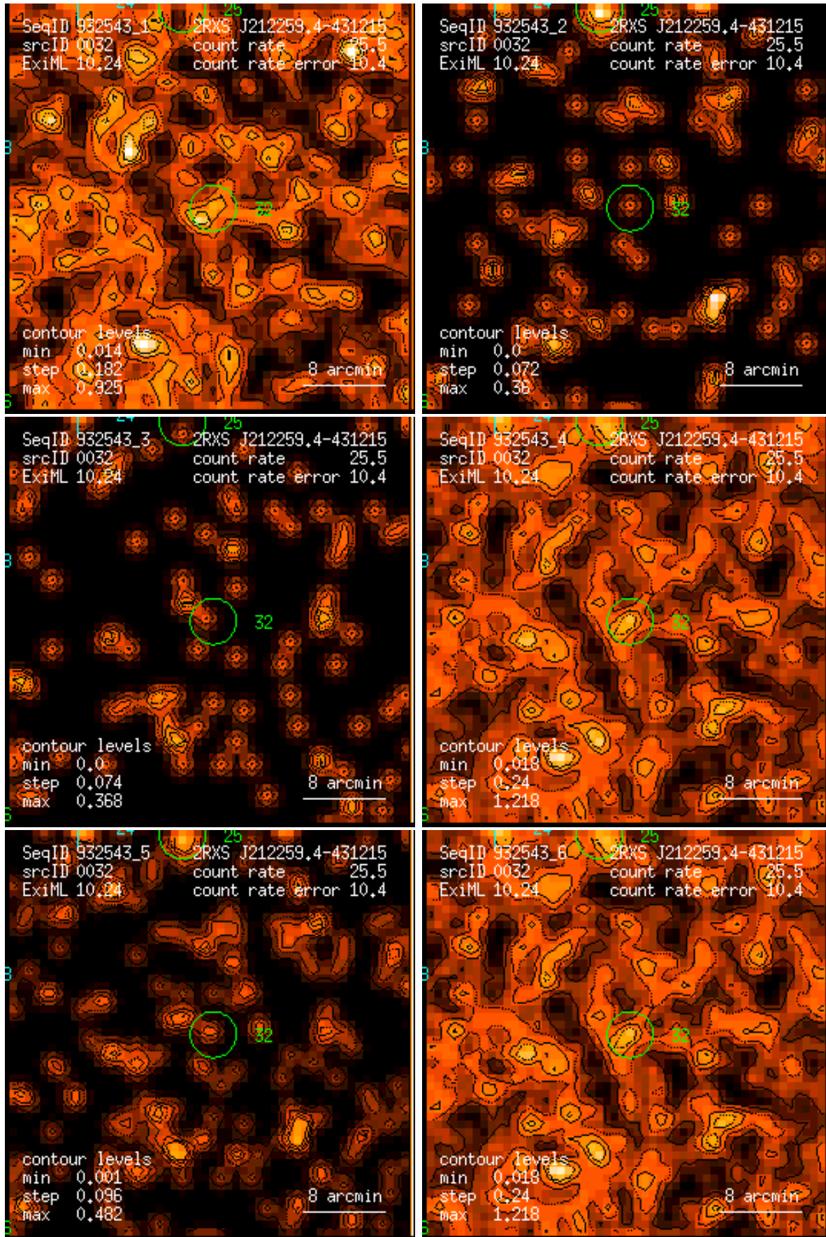
Figure 32: RASS 932543: detection 0032: band rate images, Gaussian filter: (1) PSPC channels 11 – 41, (2) 52 – 90, (3) 91 – 201, (4) 11 – 235, (5) 52 – 201, (6) 11 – 201. Broad band rates in counts/ks. Band rate contour levels in counts/ks/arcmin 2 .
