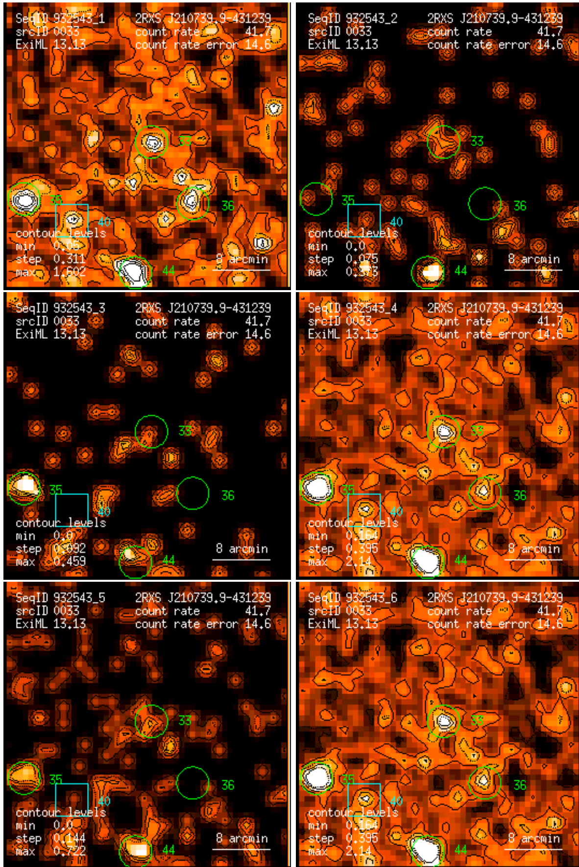
Figure 33: RASS 932543: detection 0033: band rate images, Gaussian filter: (1) PSPC channels 11 – 41, (2) 52 – 90, (3) 91 – 201, (4) 11 – 235, (5) 52 – 201, (6) 11 – 201. Broad band rates in counts/ks. Band rate contour levels in counts/ks/arcmin 2 .
