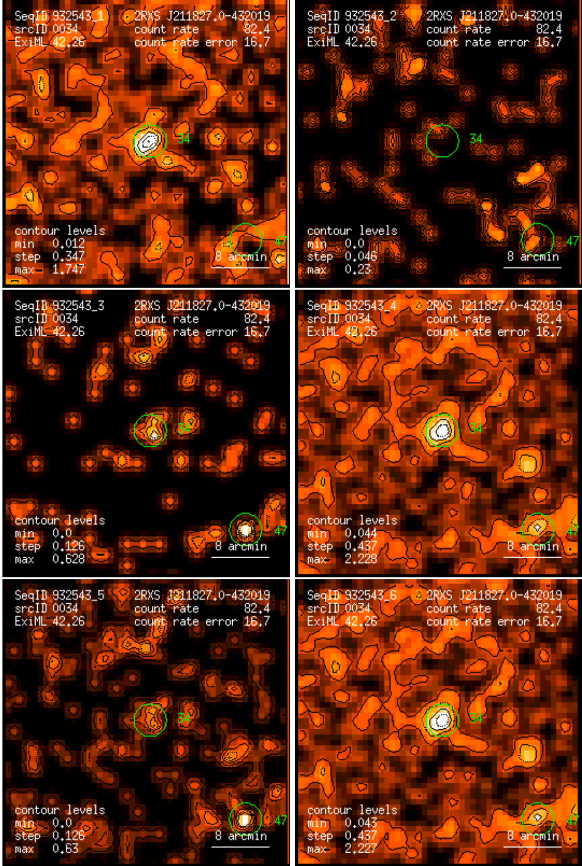
Figure 34: RASS 932543: detection 0034: band rate images, Gaussian filter: (1) PSPC channels 11 – 41, (2) 52 – 90, (3) 91 – 201, (4) 11 – 235, (5) 52 – 201, (6) 11 – 201. Broad band rates in counts/ks. Band rate contour levels in counts/ks/arcmin 2 .
