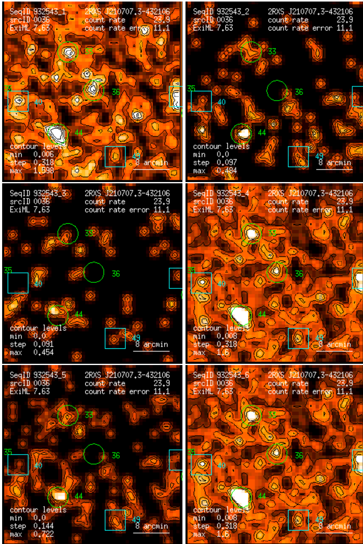
Figure 36: RASS 932543: detection 0036: band rate images, Gaussian filter: (1) PSPC channels 11 – 41, (2) 52 – 90, (3) 91 – 201, (4) 11 – 235, (5) 52 – 201, (6) 11 – 201. Broad band rates in counts/ks. Band rate contour levels in counts/ks/arcmin 2 .
