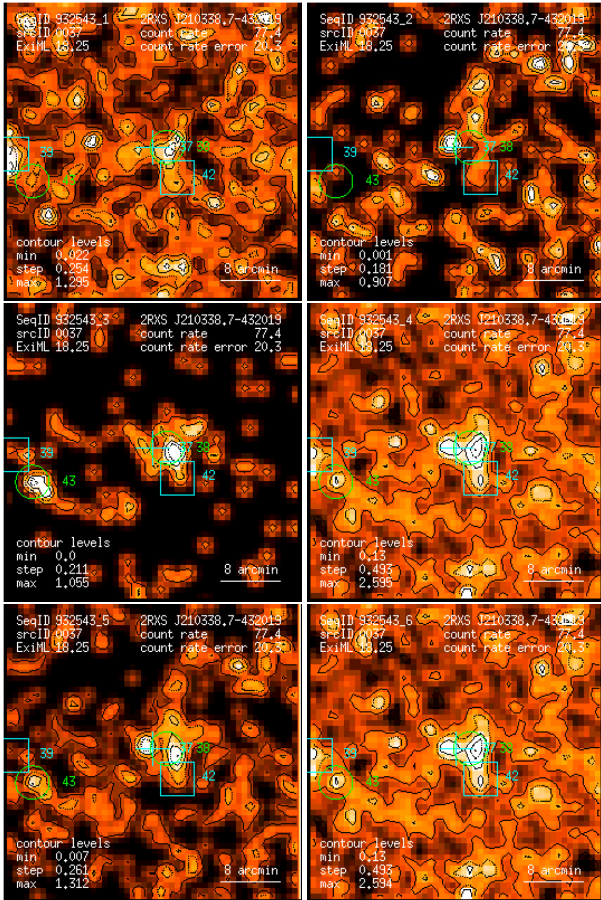
Figure 37: RASS 932543: detection 0037: band rate images, Gaussian filter: (1) PSPC channels 11 – 41, (2) 52 – 90, (3) 91 – 201, (4) 11 – 235, (5) 52 – 201, (6) 11 – 201. Broad band rates in counts/ks. Band rate contour levels in counts/ks/arcmin 2 .
