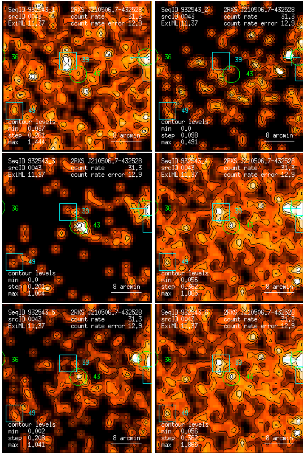
Figure 43: RASS 932543: detection 0043: band rate images, Gaussian filter: (1) PSPC channels 11 – 41, (2) 52 – 90, (3) 91 – 201, (4) 11 – 235, (5) 52 – 201, (6) 11 – 201. Broad band rates in counts/ks. Band rate contour levels in counts/ks/arcmin 2 .
