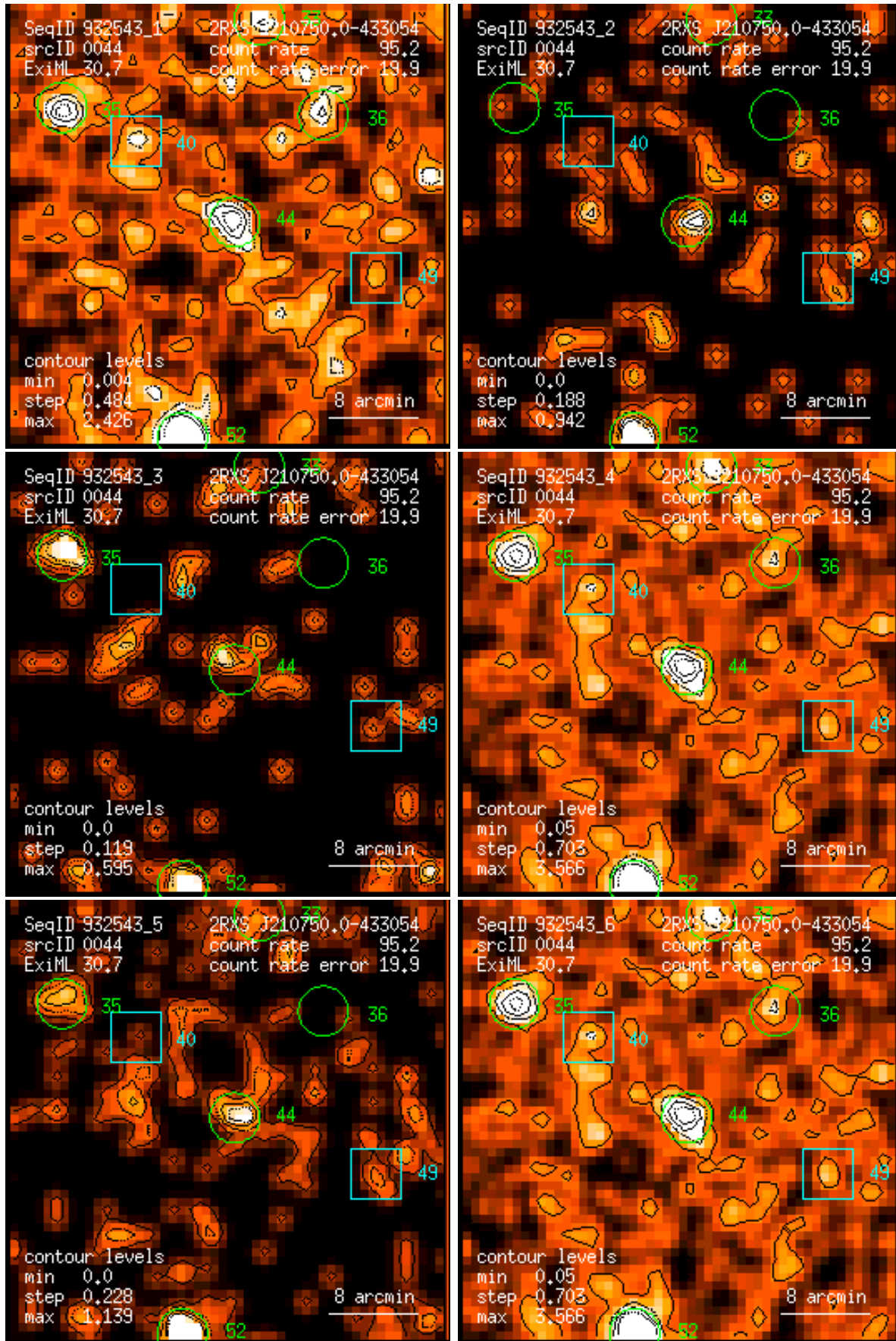
Figure 44: RASS 932543: detection 0044: band rate images, Gaussian filter: (1) PSPC channels 11 – 41, (2) 52 – 90, (3) 91 – 201, (4) 11 – 235, (5) 52 – 201, (6) 11 – 201. Broad band rates in counts/ks. Band rate contour levels in counts/ks/arcmin 2 .
