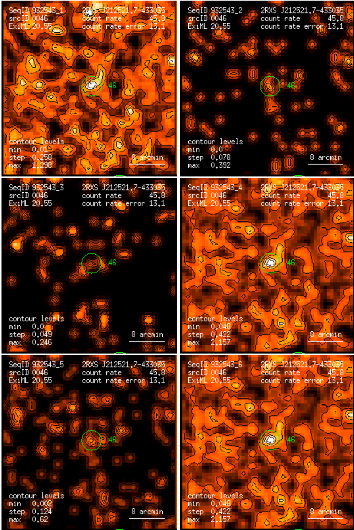
Figure 46: RASS 932543: detection 0046: band rate images, Gaussian filter: (1) PSPC channels 11 – 41, (2) 52 – 90, (3) 91 – 201, (4) 11 – 235, (5) 52 – 201, (6) 11 – 201. Broad band rates in counts/ks. Band rate contour levels in counts/ks/arcmin 2 .
