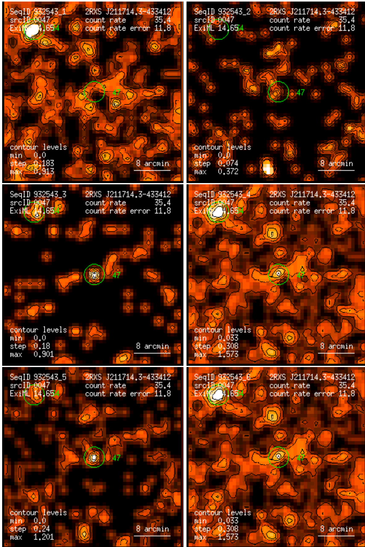
Figure 47: RASS 932543: detection 0047: band rate images, Gaussian filter: (1) PSPC channels 11 – 41, (2) 52 – 90, (3) 91 – 201, (4) 11 – 235, (5) 52 – 201, (6) 11 – 201. Broad band rates in counts/ks. Band rate contour levels in counts/ks/arcmin 2 .
