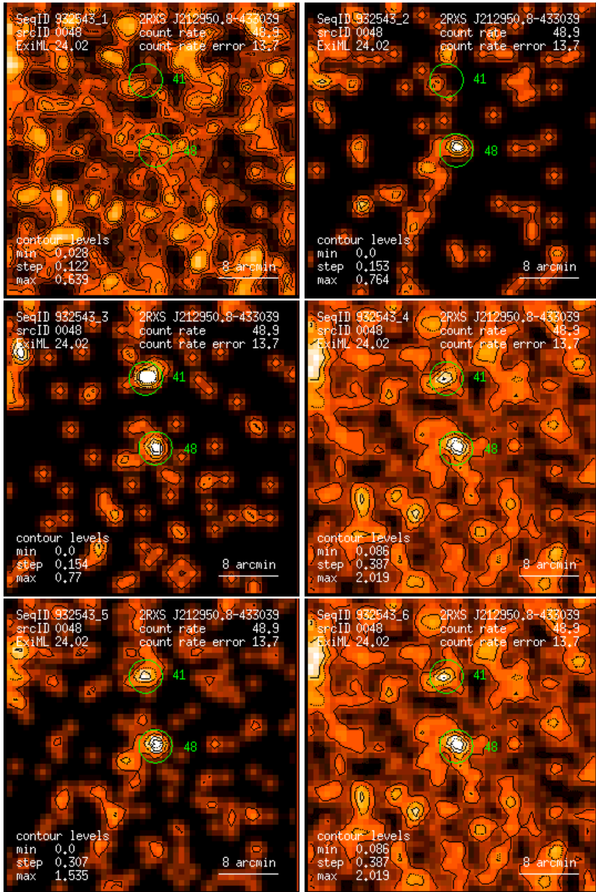
Figure 48: RASS 932543: detection 0048: band rate images, Gaussian filter: (1) PSPC channels 11 – 41, (2) 52 – 90, (3) 91 – 201, (4) 11 – 235, (5) 52 – 201, (6) 11 – 201. Broad band rates in counts/ks. Band rate contour levels in counts/ks/arcmin 2 .
