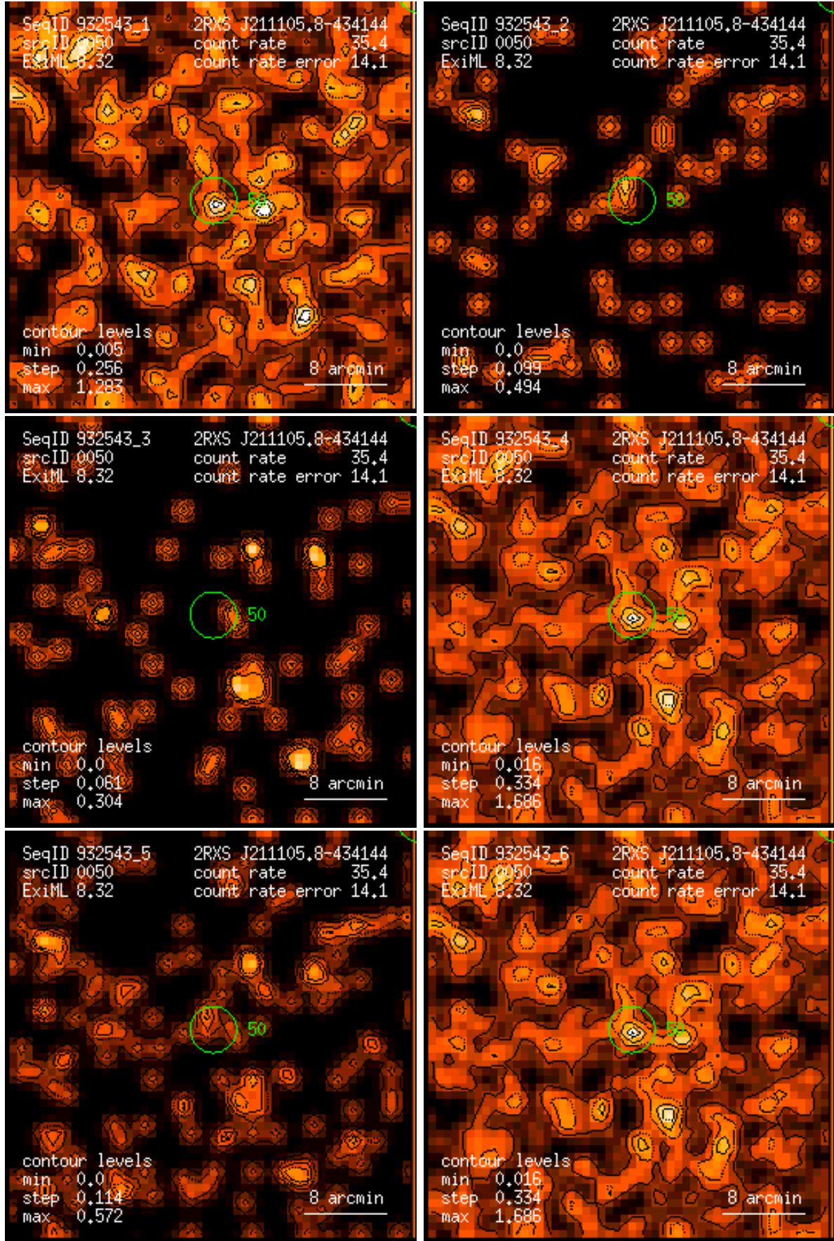
Figure 50: RASS 932543: detection 0050: band rate images, Gaussian filter: (1) PSPC channels 11 – 41, (2) 52 – 90, (3) 91 – 201, (4) 11 – 235, (5) 52 – 201, (6) 11 – 201. Broad band rates in counts/ks. Band rate contour levels in counts/ks/arcmin 2 .
