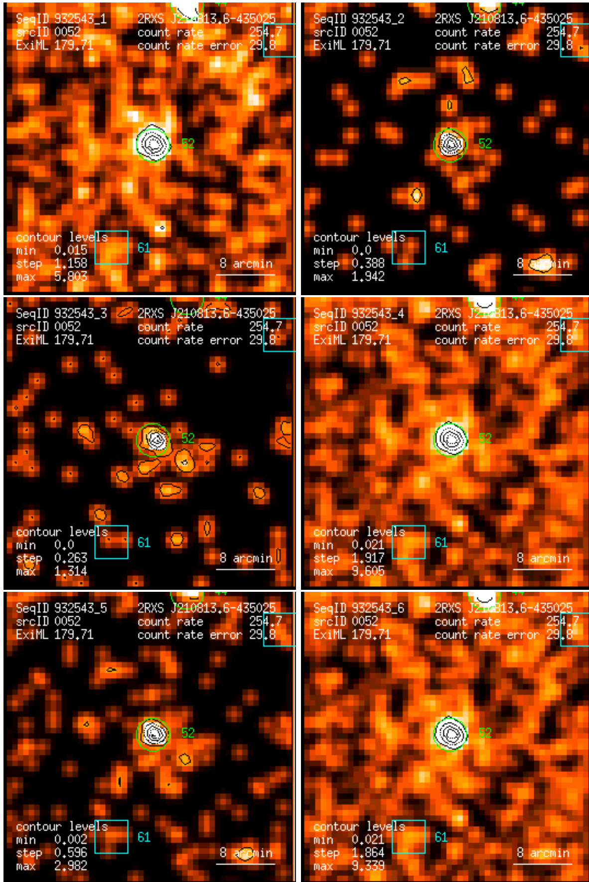
Figure 52: RASS 932543: detection 0052: band rate images, Gaussian filter: (1) PSPC channels 11 – 41, (2) 52 – 90, (3) 91 – 201, (4) 11 – 235, (5) 52 – 201, (6) 11 – 201. Broad band rates in counts/ks. Band rate contour levels in counts/ks/arcmin 2 .
