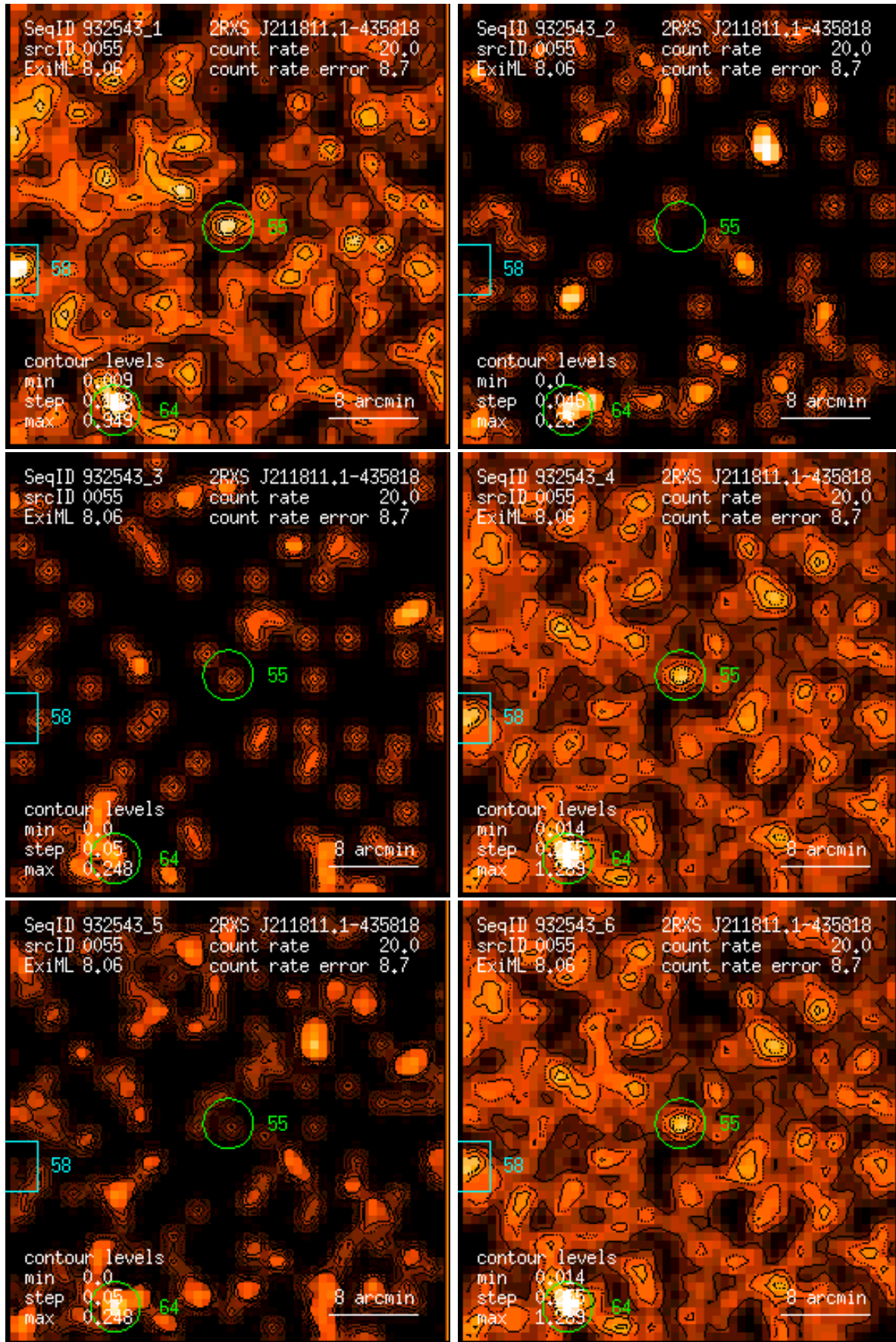
Figure 55: RASS 932543: detection 0055: band rate images, Gaussian filter: (1) PSPC channels 11 – 41, (2) 52 – 90, (3) 91 – 201, (4) 11 – 235, (5) 52 – 201, (6) 11 – 201. Broad band rates in counts/ks. Band rate contour levels in counts/ks/arcmin 2 .
