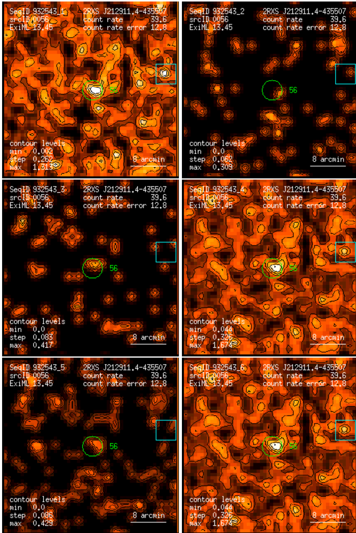
Figure 56: RASS 932543: detection 0056: band rate images, Gaussian filter: (1) PSPC channels 11 – 41, (2) 52 – 90, (3) 91 – 201, (4) 11 – 235, (5) 52 – 201, (6) 11 – 201. Broad band rates in counts/ks. Band rate contour levels in counts/ks/arcmin 2 .
