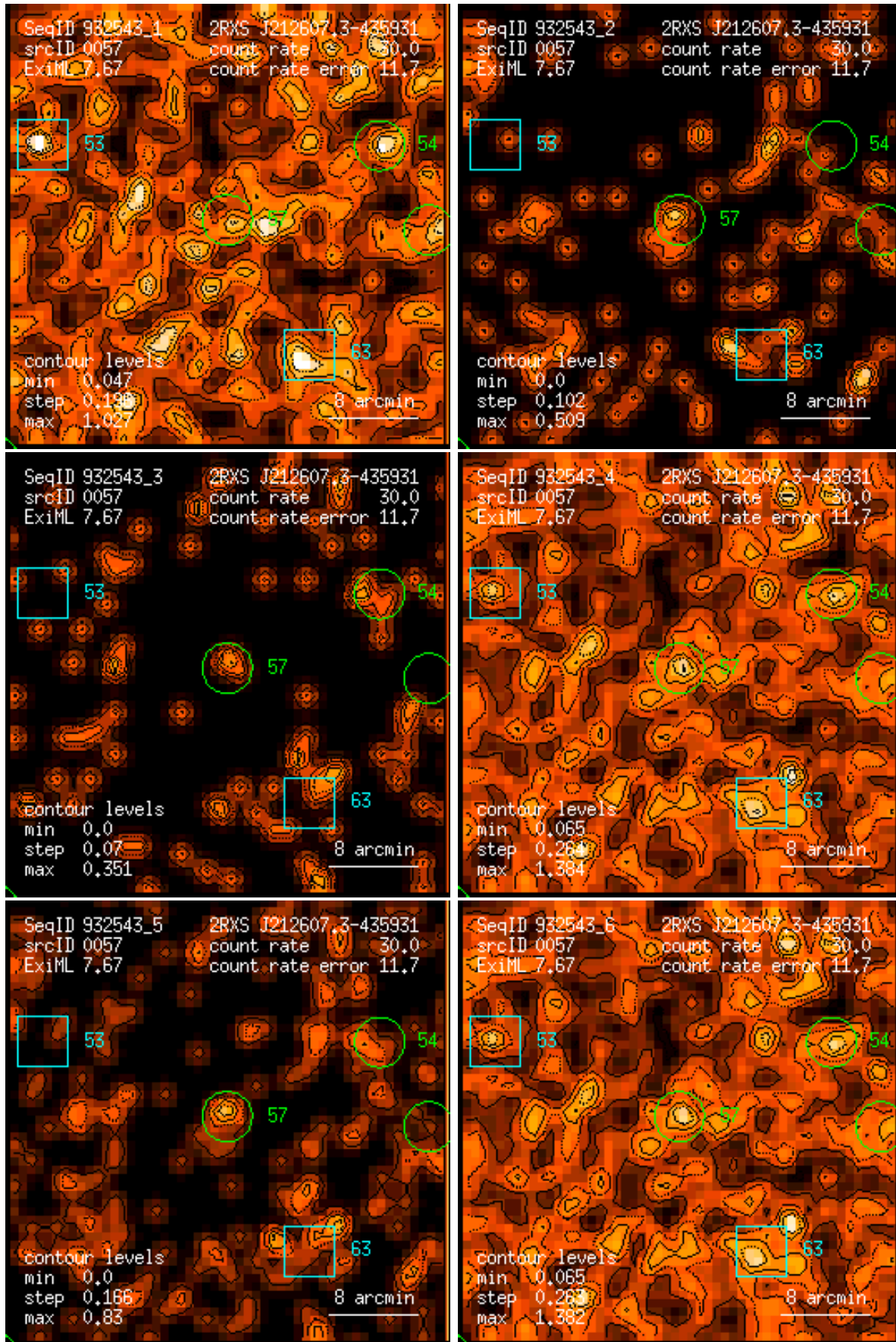
Figure 57: RASS 932543: detection 0057: band rate images, Gaussian filter: (1) PSPC channels 11 – 41, (2) 52 – 90, (3) 91 – 201, (4) 11 – 235, (5) 52 – 201, (6) 11 – 201. Broad band rates in counts/ks. Band rate contour levels in counts/ks/arcmin 2 .
