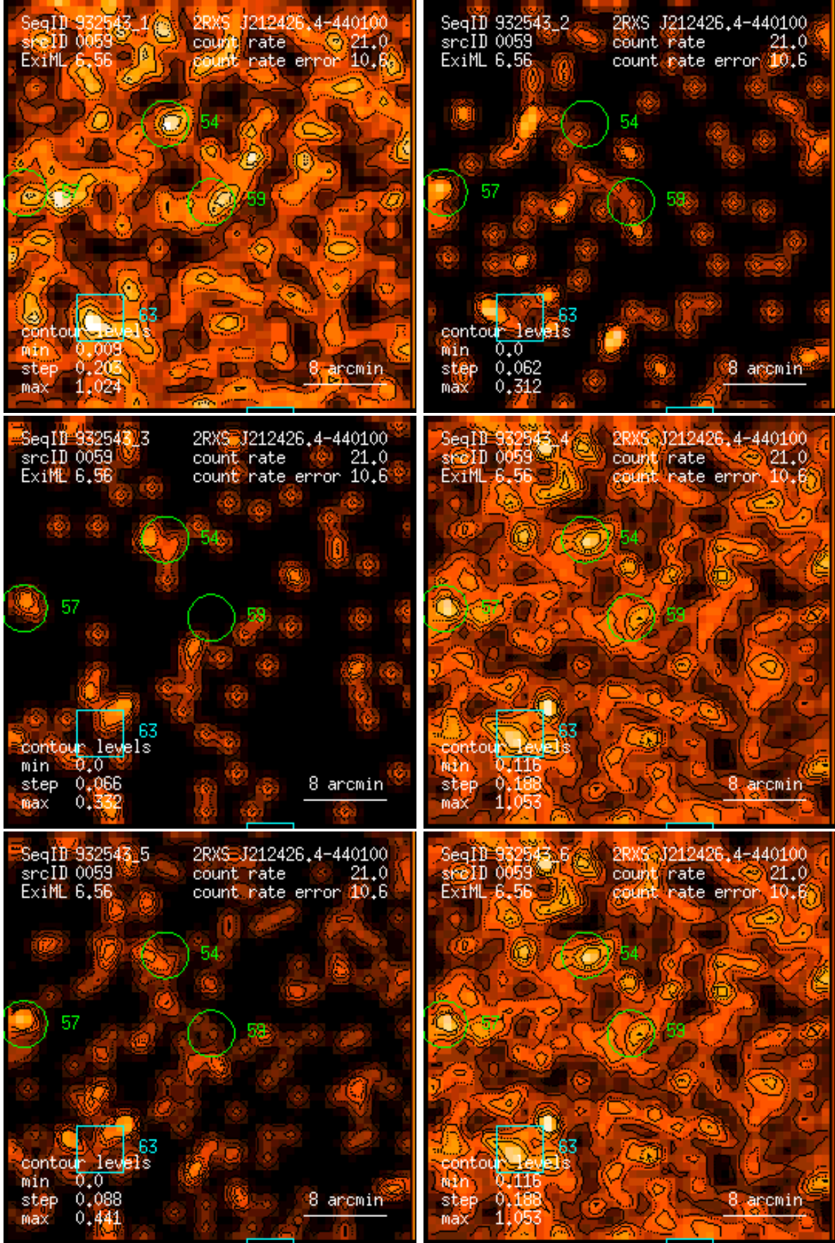
Figure 59: RASS 932543: detection 0059: band rate images, Gaussian filter: (1) PSPC channels 11 – 41, (2) 52 – 90, (3) 91 – 201, (4) 11 – 235, (5) 52 – 201, (6) 11 – 201. Broad band rates in counts/ks. Band rate contour levels in counts/ks/arcmin 2 .
