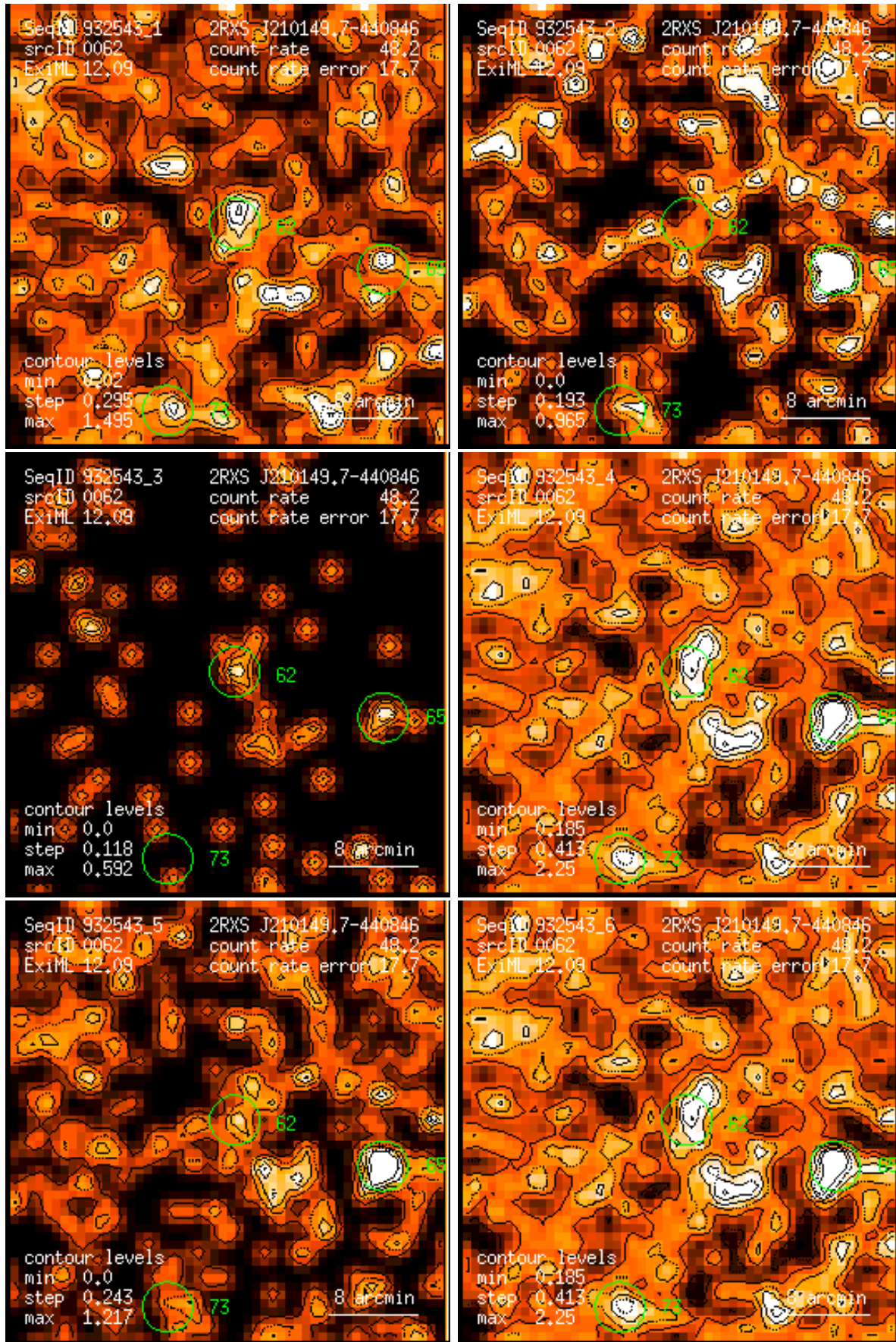
Figure 62: RASS 932543: detection 0062: band rate images, Gaussian filter: (1) PSPC channels 11 – 41, (2) 52 – 90, (3) 91 – 201, (4) 11 – 235, (5) 52 – 201, (6) 11 – 201. Broad band rates in counts/ks. Band rate contour levels in counts/ks/arcmin 2 .
