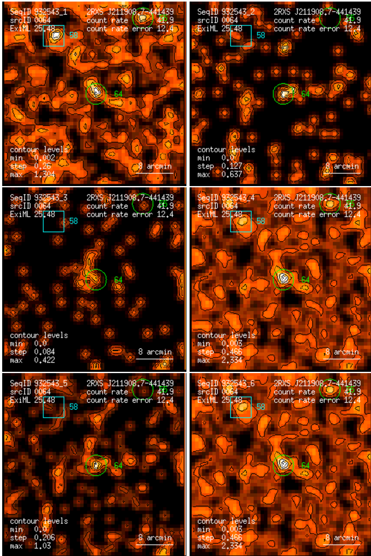
Figure 64: RASS 932543: detection 0064: band rate images, Gaussian filter: (1) PSPC channels 11 – 41, (2) 52 – 90, (3) 91 – 201, (4) 11 – 235, (5) 52 – 201, (6) 11 – 201. Broad band rates in counts/ks. Band rate contour levels in counts/ks/arcmin 2 .
