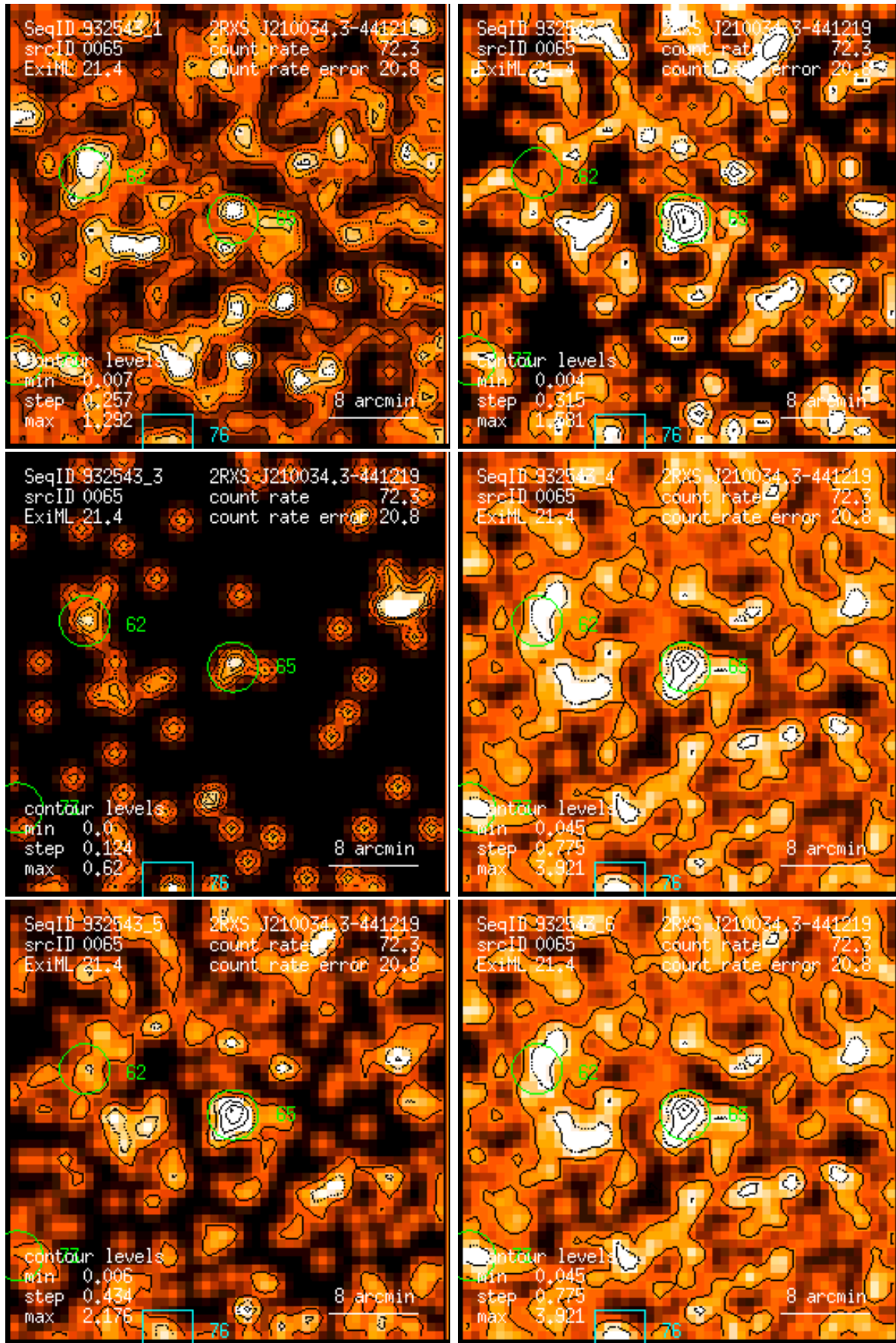
Figure 65: RASS 932543: detection 0065: band rate images, Gaussian filter: (1) PSPC channels 11 – 41, (2) 52 – 90, (3) 91 – 201, (4) 11 – 235, (5) 52 – 201, (6) 11 – 201. Broad band rates in counts/ks. Band rate contour levels in counts/ks/arcmin 2 .
