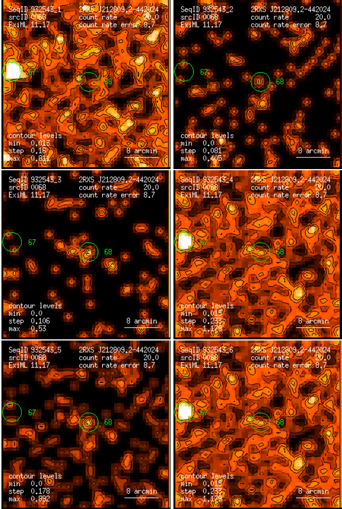
Figure 68: RASS 932543: detection 0068: band rate images, Gaussian filter: (1) PSPC channels 11 – 41, (2) 52 – 90, (3) 91 – 201, (4) 11 – 235, (5) 52 – 201, (6) 11 – 201. Broad band rates in counts/ks. Band rate contour levels in counts/ks/arcmin 2 .
