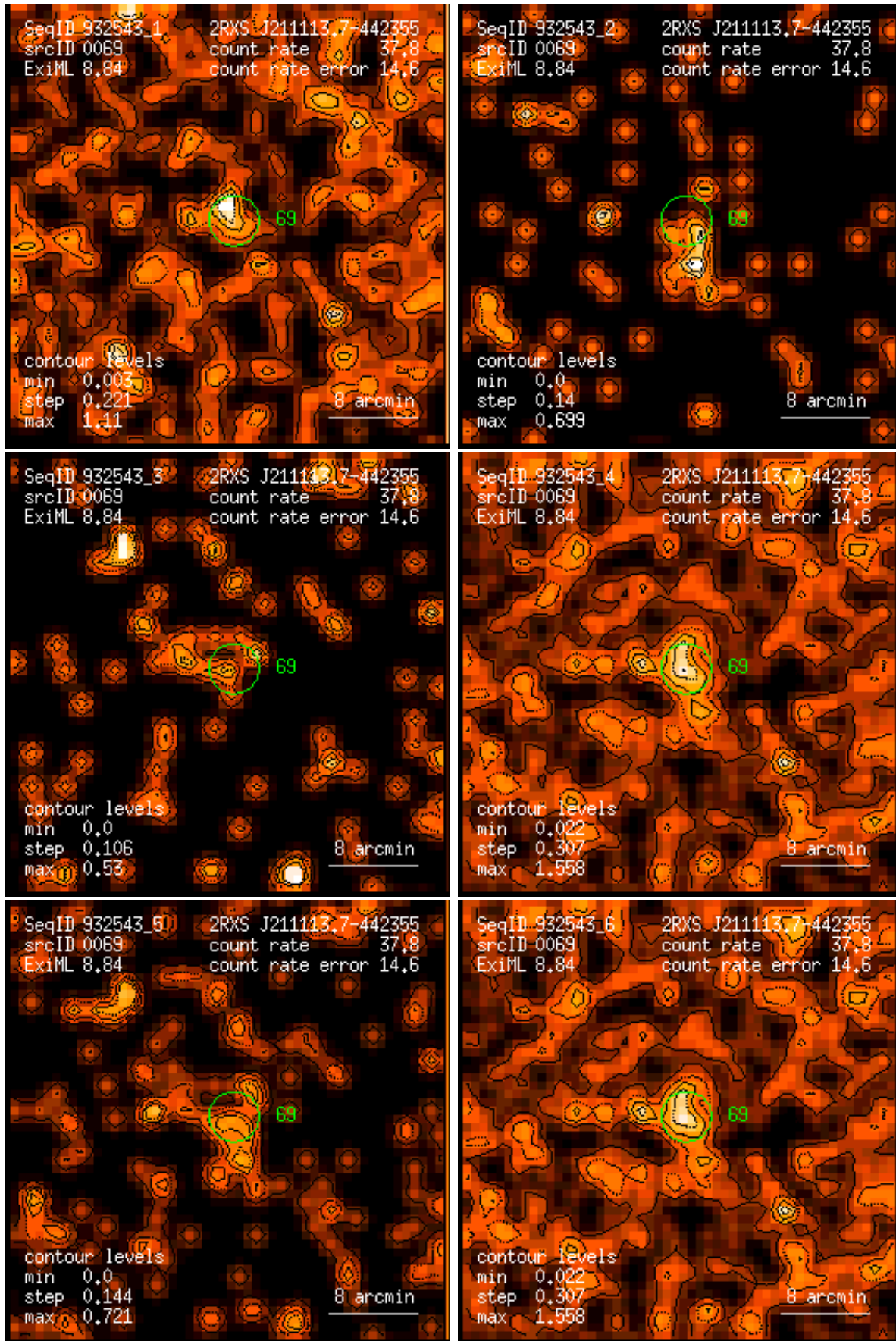
Figure 69: RASS 932543: detection 0069: band rate images, Gaussian filter: (1) PSPC channels 11 – 41, (2) 52 – 90, (3) 91 – 201, (4) 11 – 235, (5) 52 – 201, (6) 11 – 201. Broad band rates in counts/ks. Band rate contour levels in counts/ks/arcmin 2 .
