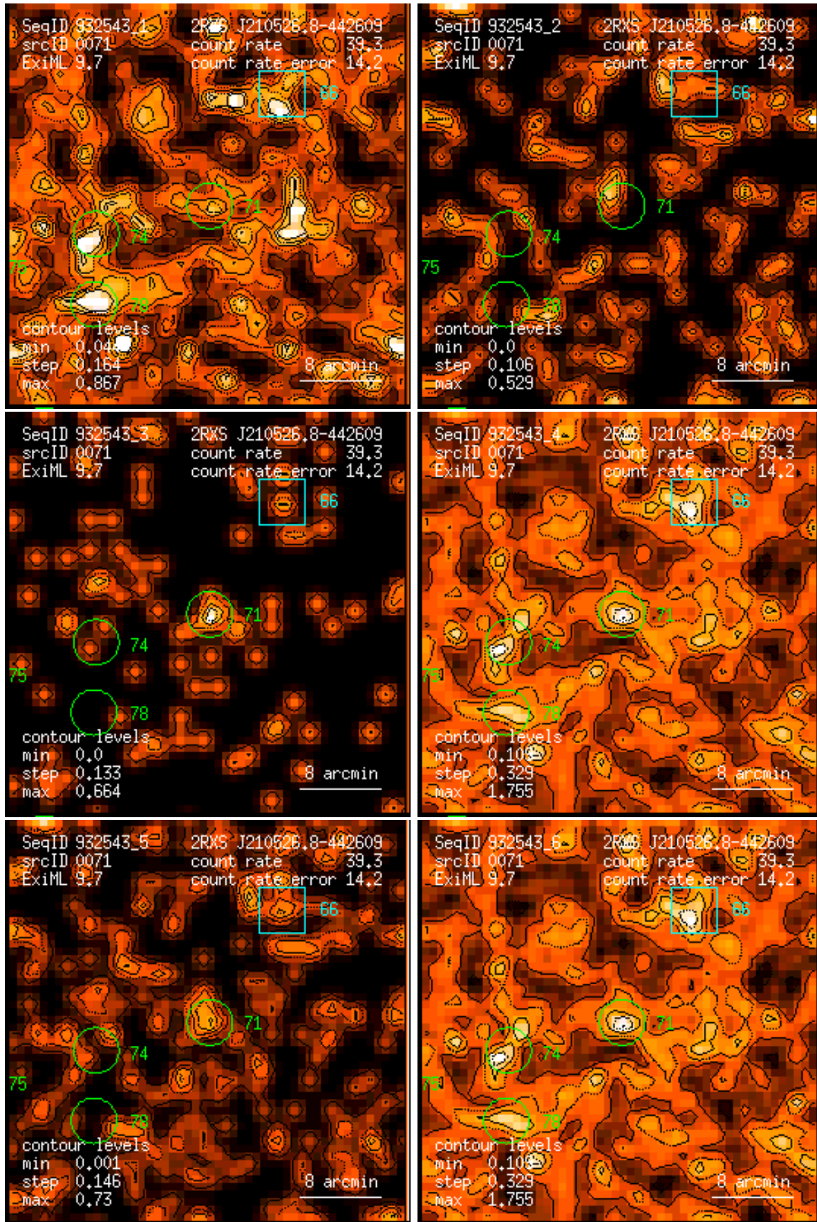
Figure 71: RASS 932543: detection 0071: band rate images, Gaussian filter: (1) PSPC channels 11 – 41, (2) 52 – 90, (3) 91 – 201, (4) 11 – 235, (5) 52 – 201, (6) 11 – 201. Broad band rates in counts/ks. Band rate contour levels in counts/ks/arcmin 2 .
