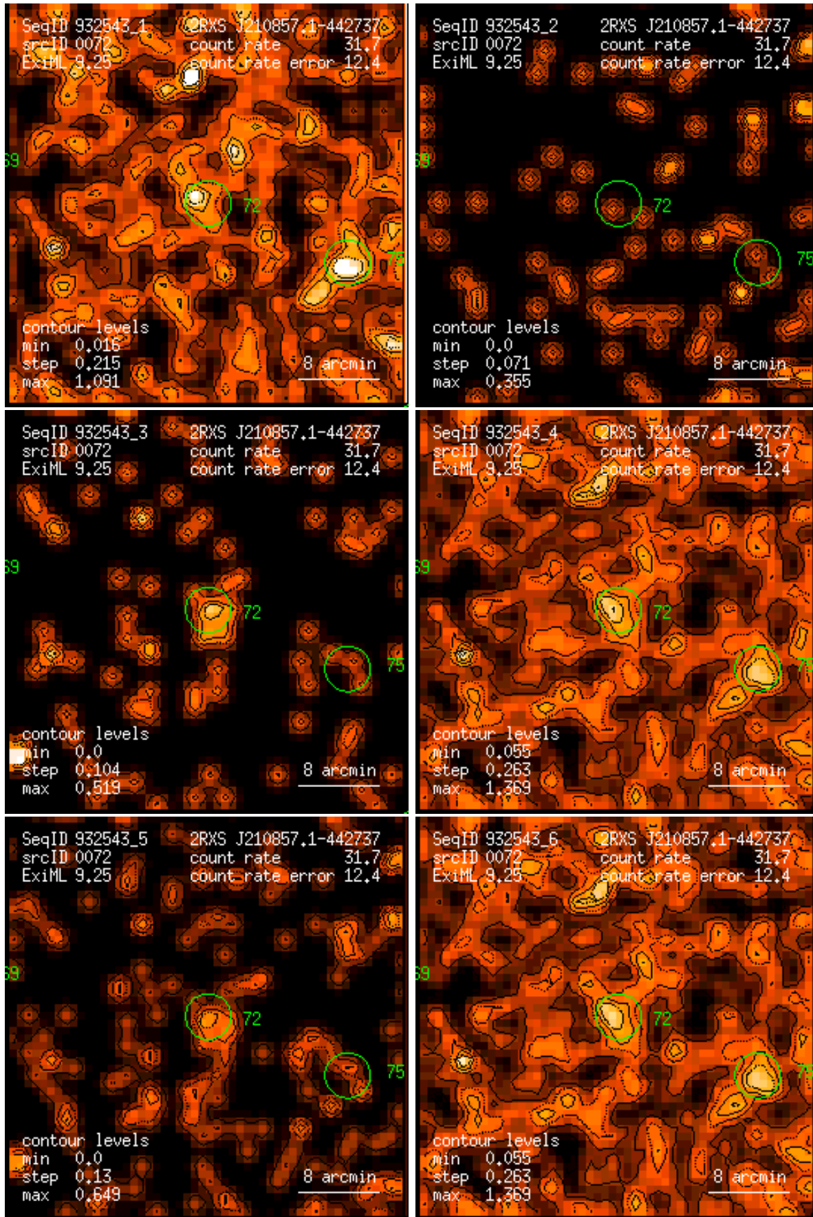
Figure 72: RASS 932543: detection 0072: band rate images, Gaussian filter: (1) PSPC channels 11 – 41, (2) 52 – 90, (3) 91 – 201, (4) 11 – 235, (5) 52 – 201, (6) 11 – 201. Broad band rates in counts/ks. Band rate contour levels in counts/ks/arcmin 2 .
