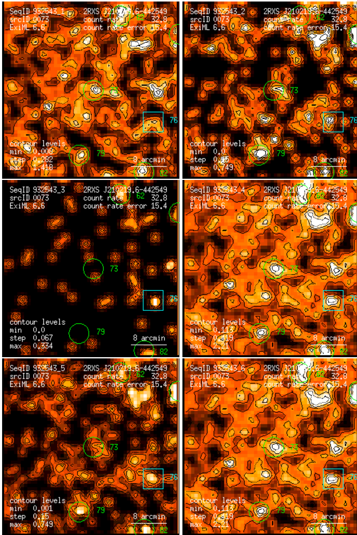
Figure 73: RASS 932543: detection 0073: band rate images, Gaussian filter: (1) PSPC channels 11 – 41, (2) 52 – 90, (3) 91 – 201, (4) 11 – 235, (5) 52 – 201, (6) 11 – 201. Broad band rates in counts/ks. Band rate contour levels in counts/ks/arcmin 2 .
