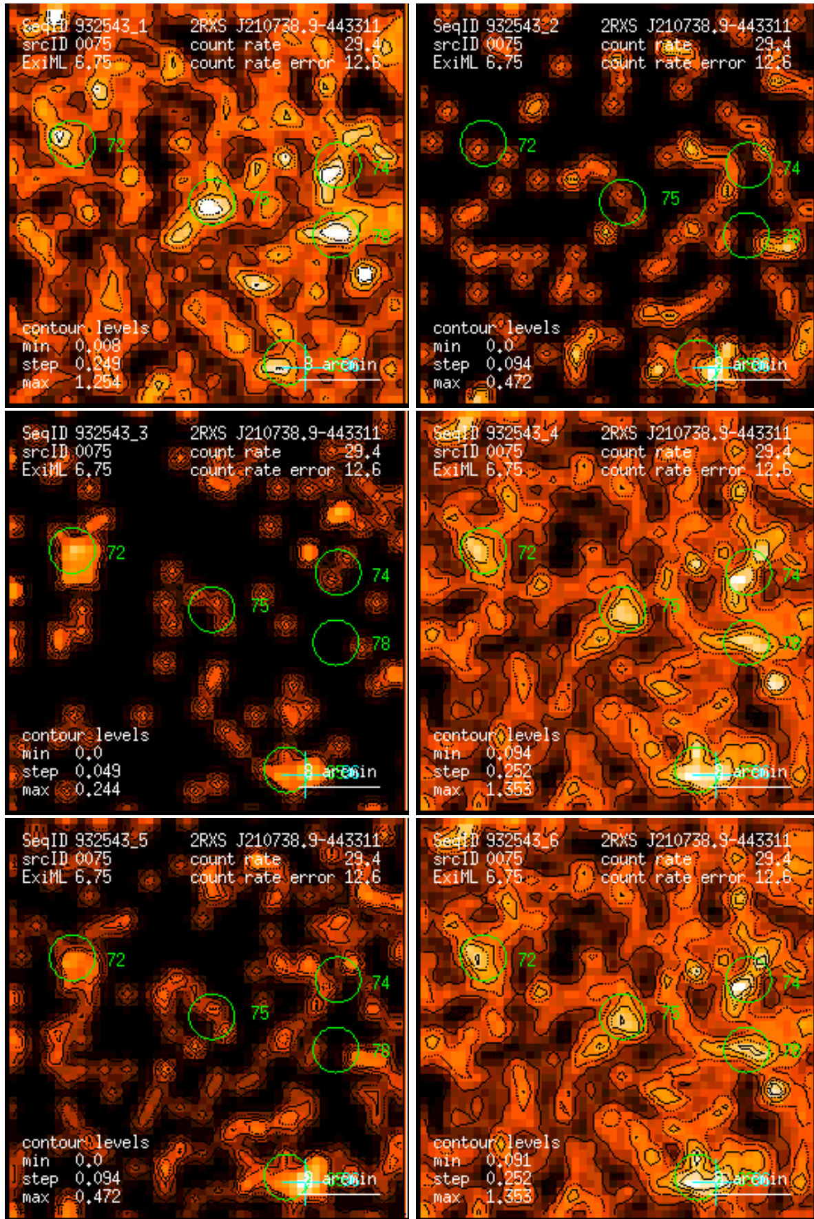
Figure 75: RASS 932543: detection 0075: band rate images, Gaussian filter: (1) PSPC channels 11 – 41, (2) 52 – 90, (3) 91 – 201, (4) 11 – 235, (5) 52 – 201, (6) 11 – 201. Broad band rates in counts/ks. Band rate contour levels in counts/ks/arcmin 2 .
