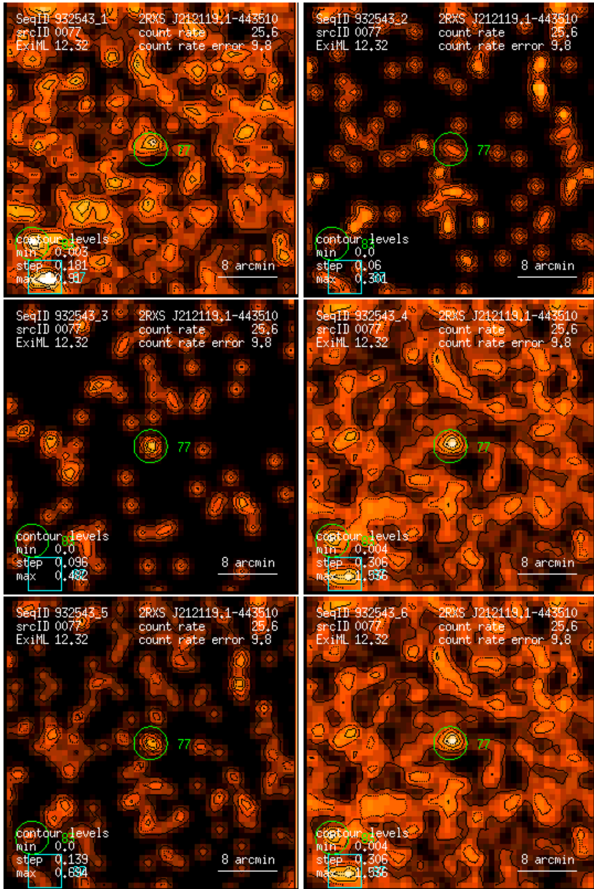
Figure 77: RASS 932543: detection 0077: band rate images, Gaussian filter: (1) PSPC channels 11 – 41, (2) 52 – 90, (3) 91 – 201, (4) 11 – 235, (5) 52 – 201, (6) 11 – 201. Broad band rates in counts/ks. Band rate contour levels in counts/ks/arcmin 2 .
