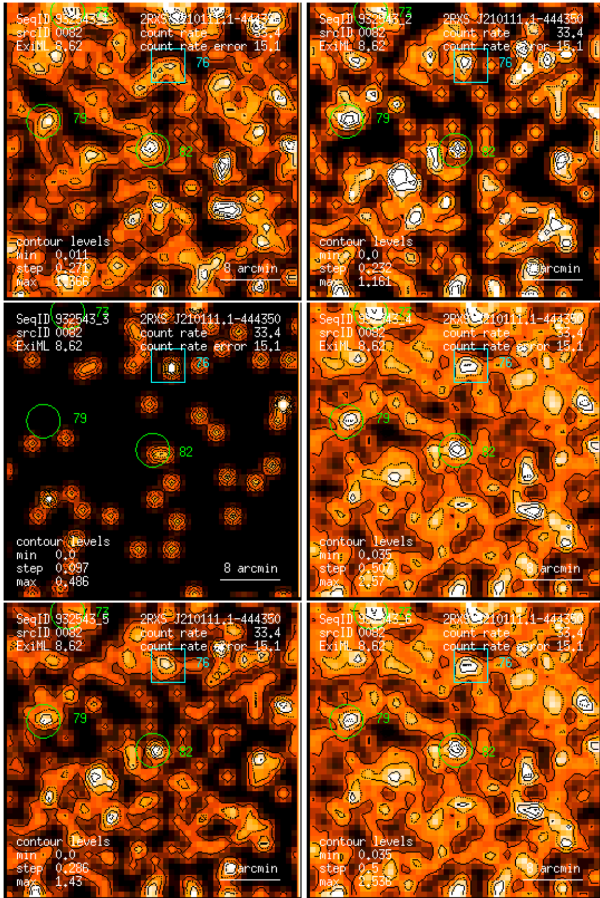
Figure 82: RASS 932543: detection 0082: band rate images, Gaussian filter: (1) PSPC channels 11 – 41, (2) 52 – 90, (3) 91 – 201, (4) 11 – 235, (5) 52 – 201, (6) 11 – 201. Broad band rates in counts/ks. Band rate contour levels in counts/ks/arcmin 2 .
