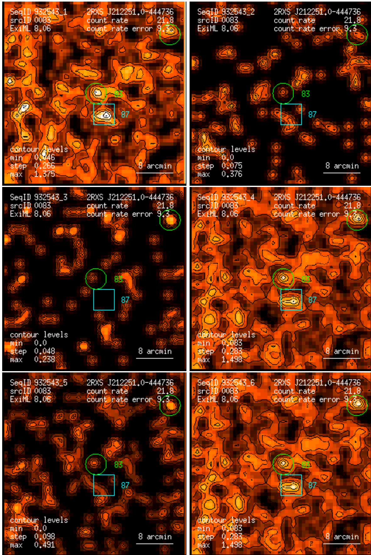
Figure 83: RASS 932543: detection 0083: band rate images, Gaussian filter: (1) PSPC channels 11 – 41, (2) 52 – 90, (3) 91 – 201, (4) 11 – 235, (5) 52 – 201, (6) 11 – 201. Broad band rates in counts/ks. Band rate contour levels in counts/ks/arcmin 2 .
