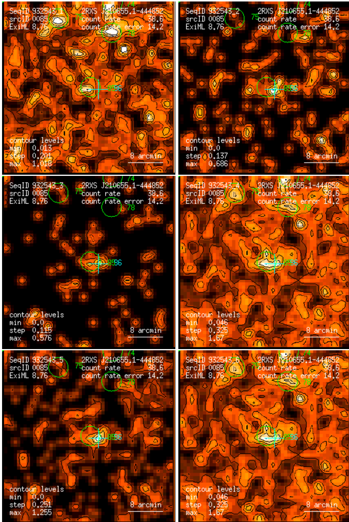
Figure 85: RASS 932543: detection 0085: band rate images, Gaussian filter: (1) PSPC channels 11 – 41, (2) 52 – 90, (3) 91 – 201, (4) 11 – 235, (5) 52 – 201, (6) 11 – 201. Broad band rates in counts/ks. Band rate contour levels in counts/ks/arcmin 2 .
