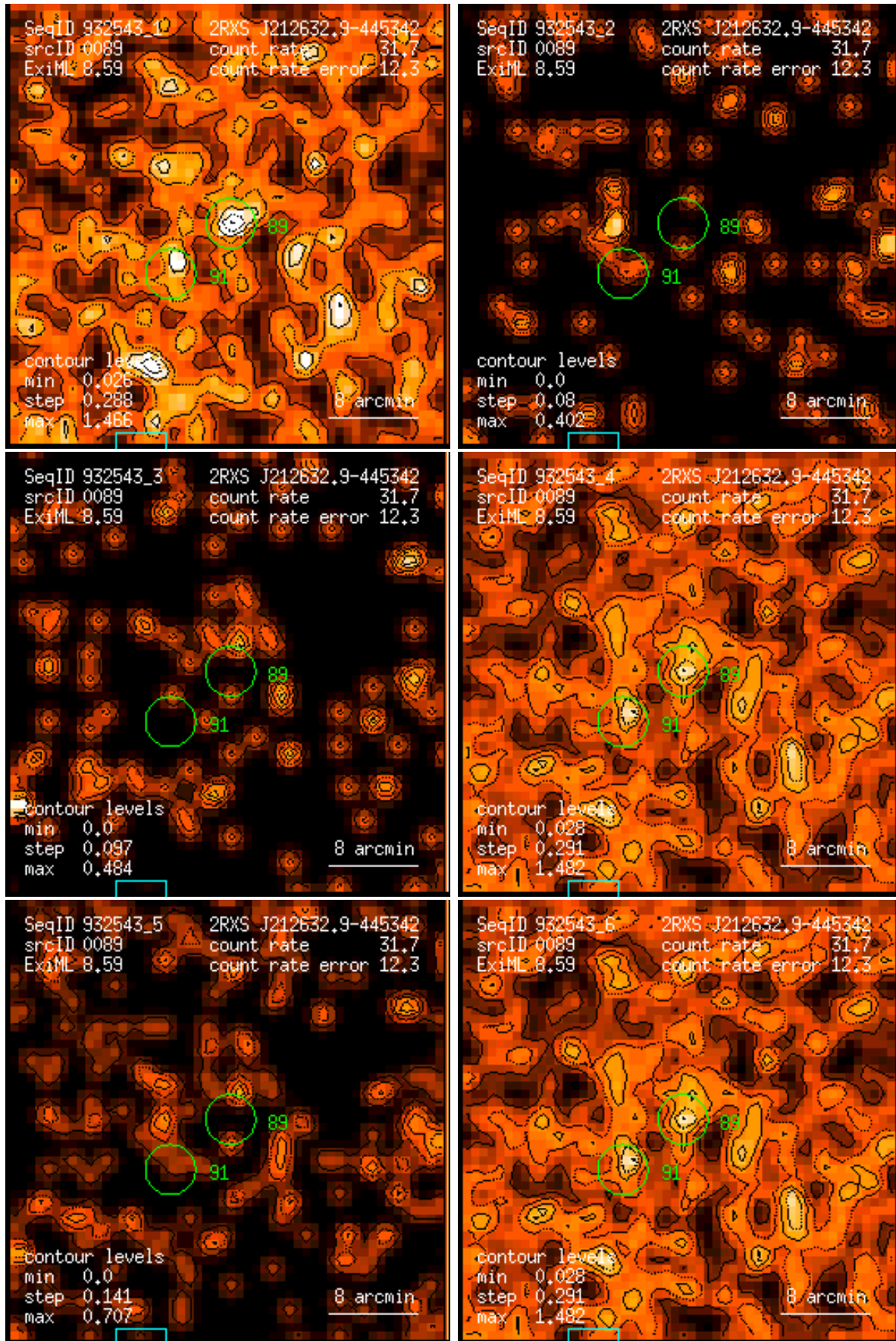
Figure 89: RASS 932543: detection 0089: band rate images, Gaussian filter: (1) PSPC channels 11 – 41, (2) 52 – 90, (3) 91 – 201, (4) 11 – 235, (5) 52 – 201, (6) 11 – 201. Broad band rates in counts/ks. Band rate contour levels in counts/ks/arcmin 2 .
