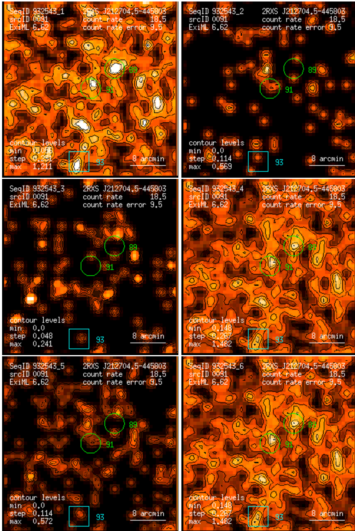
Figure 91: RASS 932543: detection 0091: band rate images, Gaussian filter: (1) PSPC channels 11 – 41, (2) 52 – 90, (3) 91 – 201, (4) 11 – 235, (5) 52 – 201, (6) 11 – 201. Broad band rates in counts/ks. Band rate contour levels in counts/ks/arcmin 2 .
