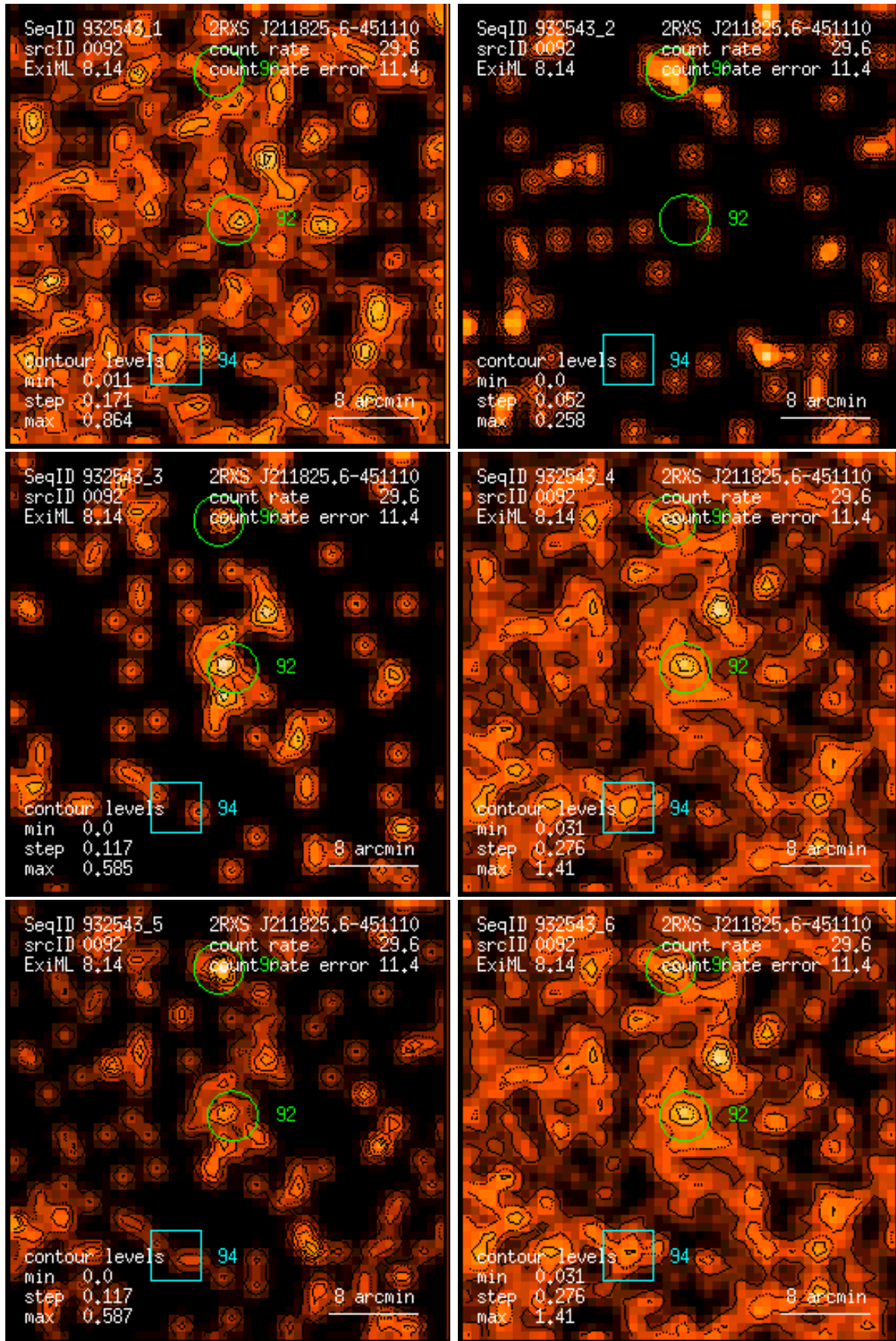
Figure 92: RASS 932543: detection 0092: band rate images, Gaussian filter: (1) PSPC channels 11 – 41, (2) 52 – 90, (3) 91 – 201, (4) 11 – 235, (5) 52 – 201, (6) 11 – 201. Broad band rates in counts/ks. Band rate contour levels in counts/ks/arcmin 2 .
