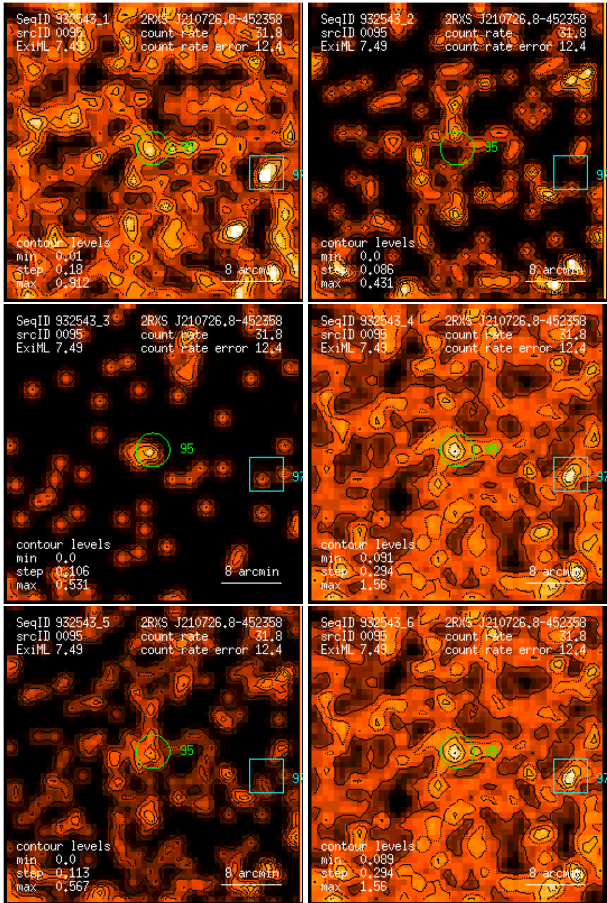
Figure 95: RASS 932543: detection 0095: band rate images, Gaussian filter: (1) PSPC channels 11 – 41, (2) 52 – 90, (3) 91 – 201, (4) 11 – 235, (5) 52 – 201, (6) 11 – 201. Broad band rates in counts/ks. Band rate contour levels in counts/ks/arcmin 2 .
