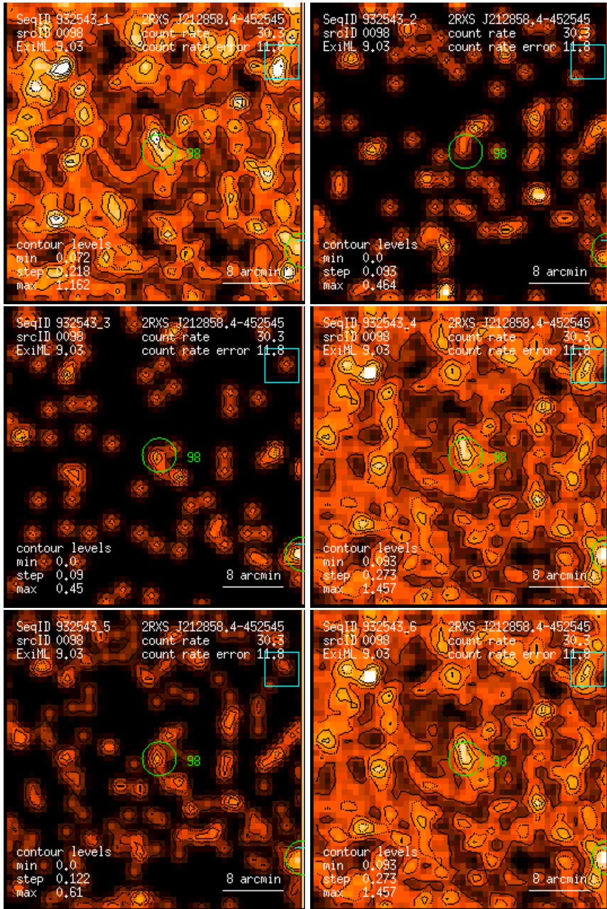
Figure 98: RASS 932543: detection 0098: band rate images, Gaussian filter: (1) PSPC channels 11 – 41, (2) 52 – 90, (3) 91 – 201, (4) 11 – 235, (5) 52 – 201, (6) 11 – 201. Broad band rates in counts/ks. Band rate contour levels in counts/ks/arcmin 2 .
