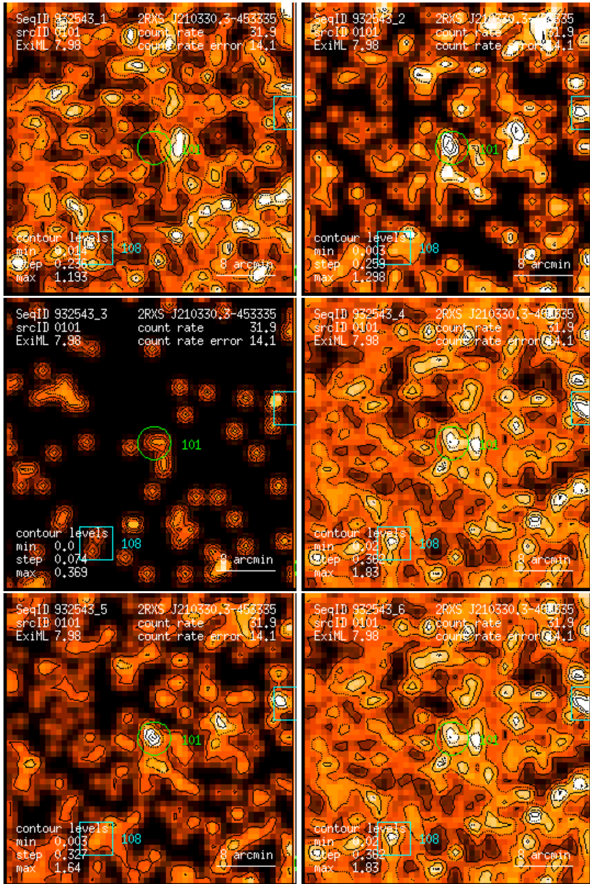
Figure 101: RASS 932543: detection 0101: band rate images, Gaussian filter: (1) PSPC channels 11 – 41, (2) 52 – 90, (3) 91 – 201, (4) 11 – 235, (5) 52 – 201, (6) 11 – 201. Broad band rates in counts/ks. Band rate contour levels in counts/ks/arcmin 2 .
