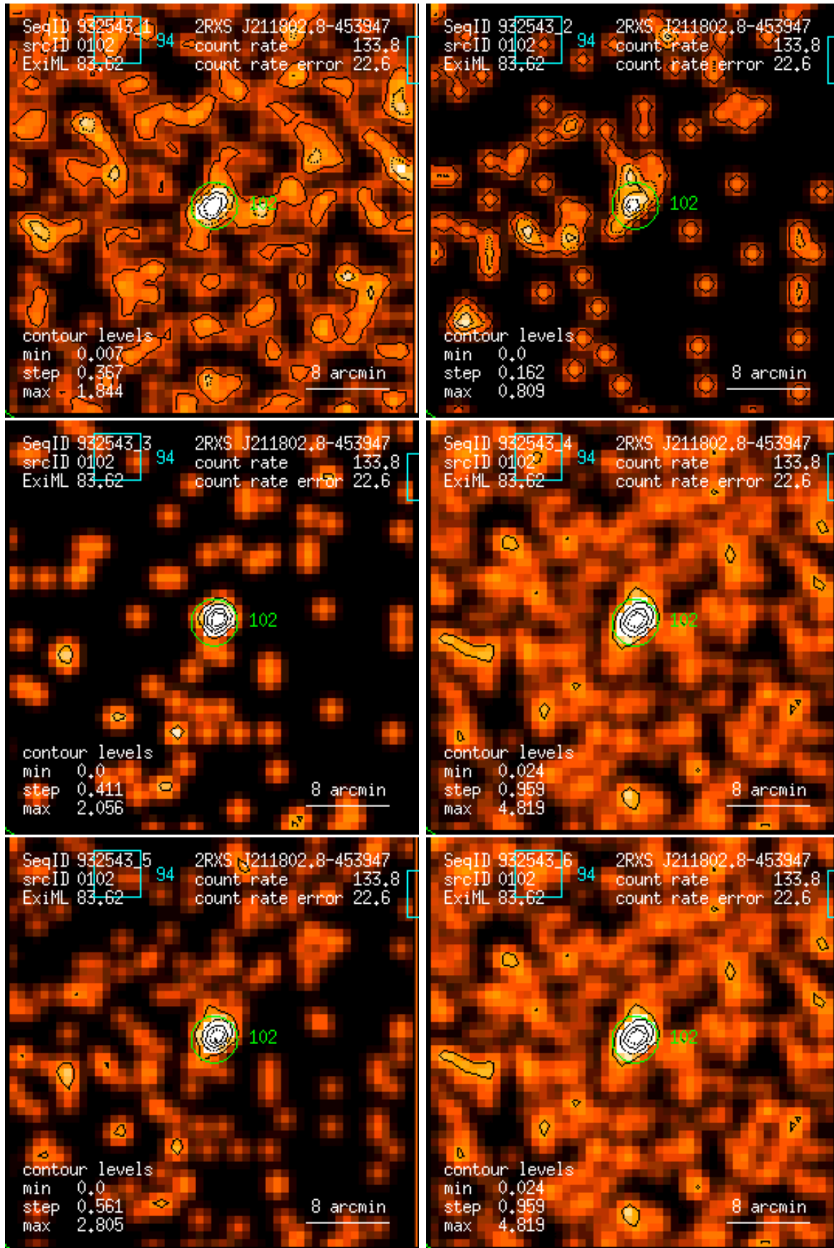
Figure 102: RASS 932543: detection 0102: band rate images, Gaussian filter: (1) PSPC channels 11 – 41, (2) 52 – 90, (3) 91 – 201, (4) 11 – 235, (5) 52 – 201, (6) 11 – 201. Broad band rates in counts/ks. Band rate contour levels in counts/ks/arcmin 2 .
