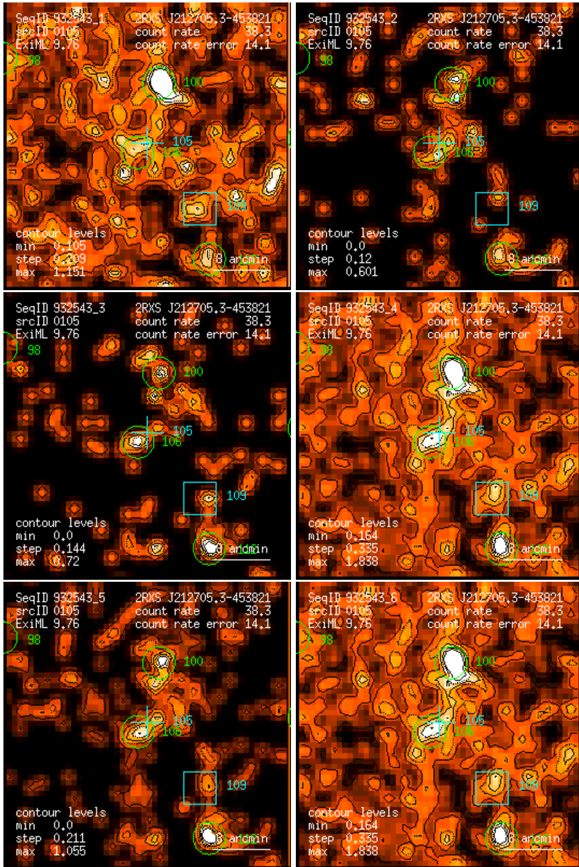
Figure 105: RASS 932543: detection 0105: band rate images, Gaussian filter: (1) PSPC channels 11 – 41, (2) 52 – 90, (3) 91 – 201, (4) 11 – 235, (5) 52 – 201, (6) 11 – 201. Broad band rates in counts/ks. Band rate contour levels in counts/ks/arcmin 2 .
