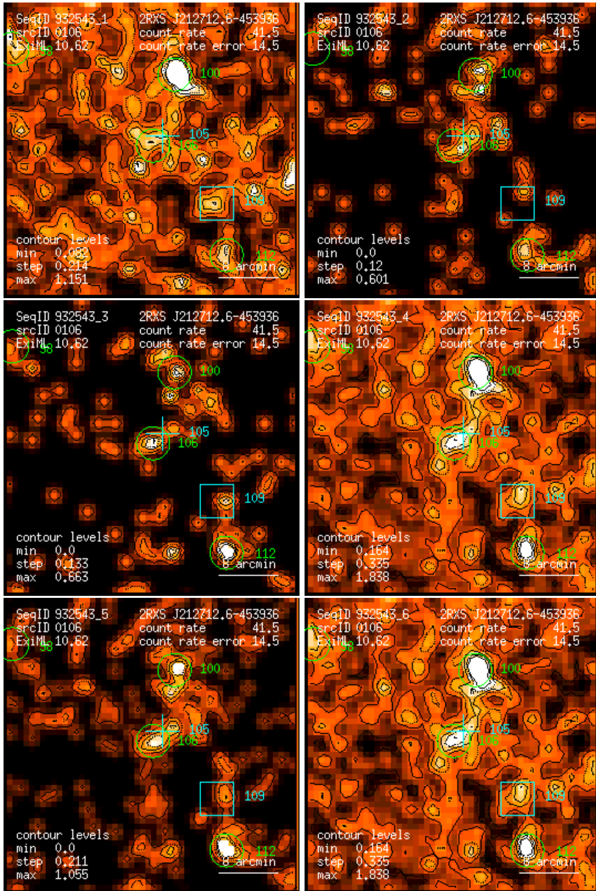
Figure 106: RASS 932543: detection 0106: band rate images, Gaussian filter: (1) PSPC channels 11 – 41, (2) 52 – 90, (3) 91 – 201, (4) 11 – 235, (5) 52 – 201, (6) 11 – 201. Broad band rates in counts/ks. Band rate contour levels in counts/ks/arcmin 2 .
