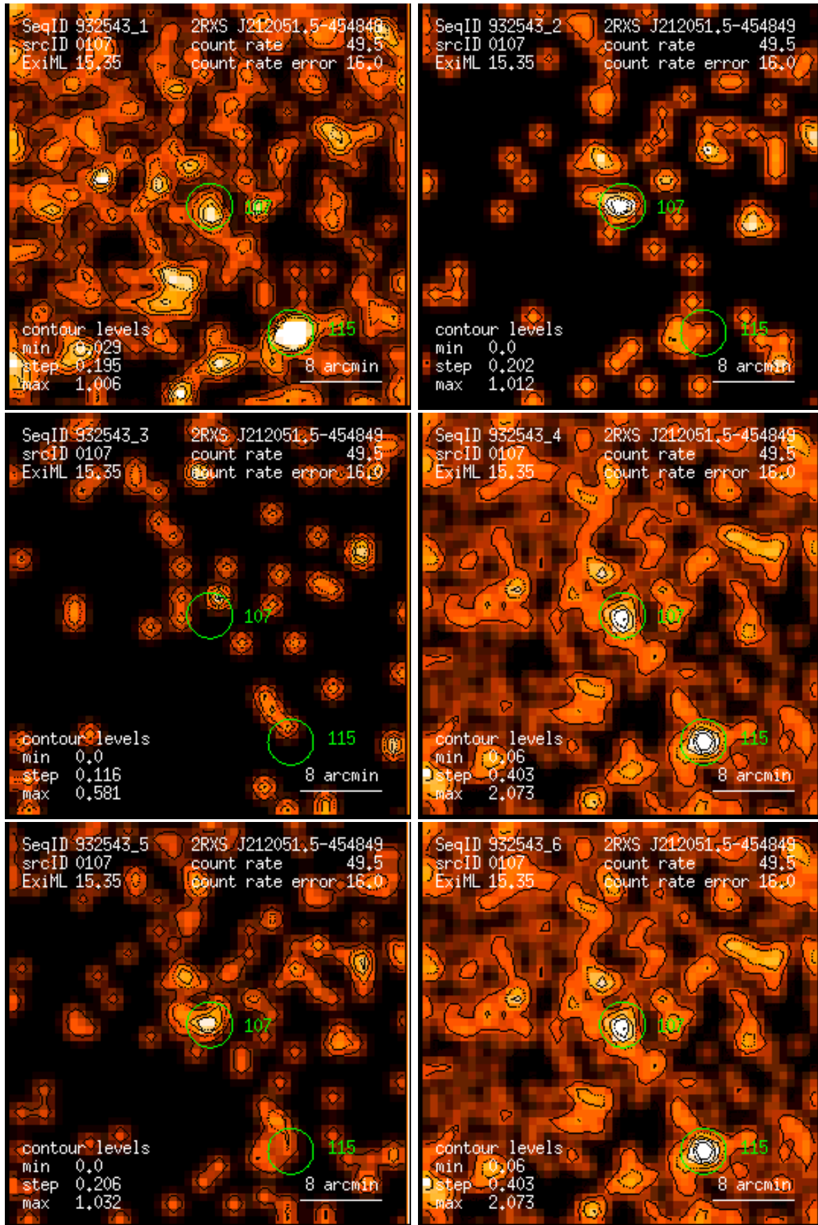
Figure 107: RASS 932543: detection 0107: band rate images, Gaussian filter: (1) PSPC channels 11 – 41, (2) 52 – 90, (3) 91 – 201, (4) 11 – 235, (5) 52 – 201, (6) 11 – 201. Broad band rates in counts/ks. Band rate contour levels in counts/ks/arcmin 2 .
