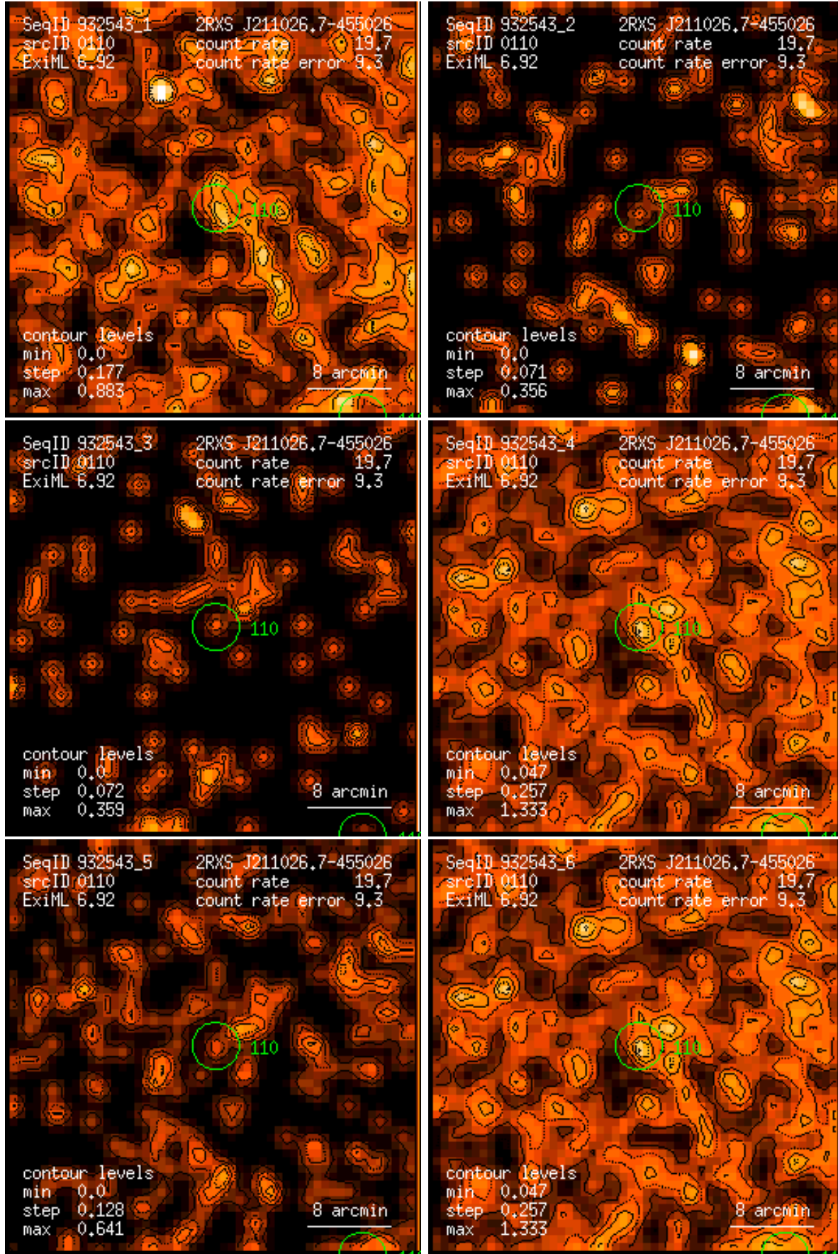
Figure 110: RASS 932543: detection 0110: band rate images, Gaussian filter: (1) PSPC channels 11 – 41, (2) 52 – 90, (3) 91 – 201, (4) 11 – 235, (5) 52 – 201, (6) 11 – 201. Broad band rates in counts/ks. Band rate contour levels in counts/ks/arcmin 2 .
